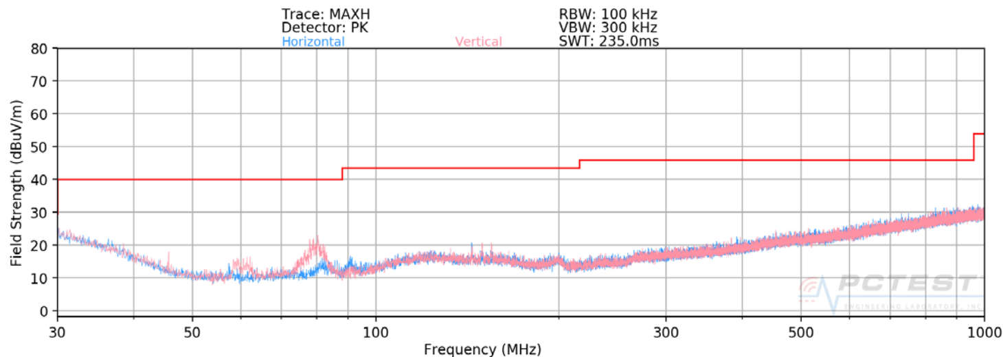
Plot 7-48. Radiated Spurious Plot below 1GHz
