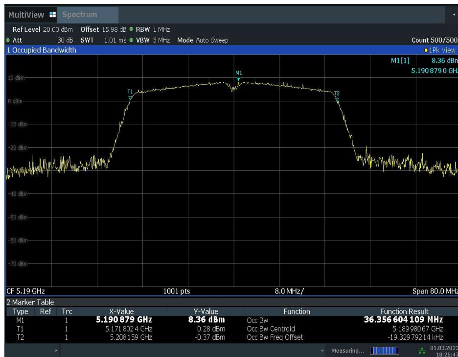
Fig.39 99% Occupied bandwidth (802.11ac-HT40, 5190MHz)
