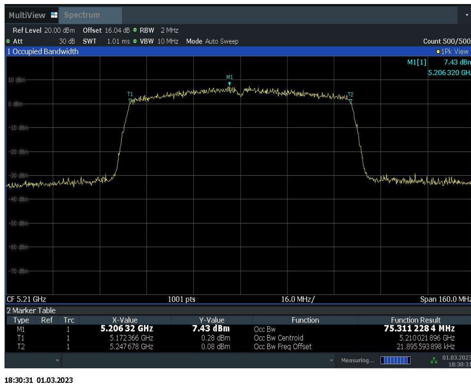
Fig.41 99% Occupied bandwidth (802.11ac-HT80, 5210MHz)
