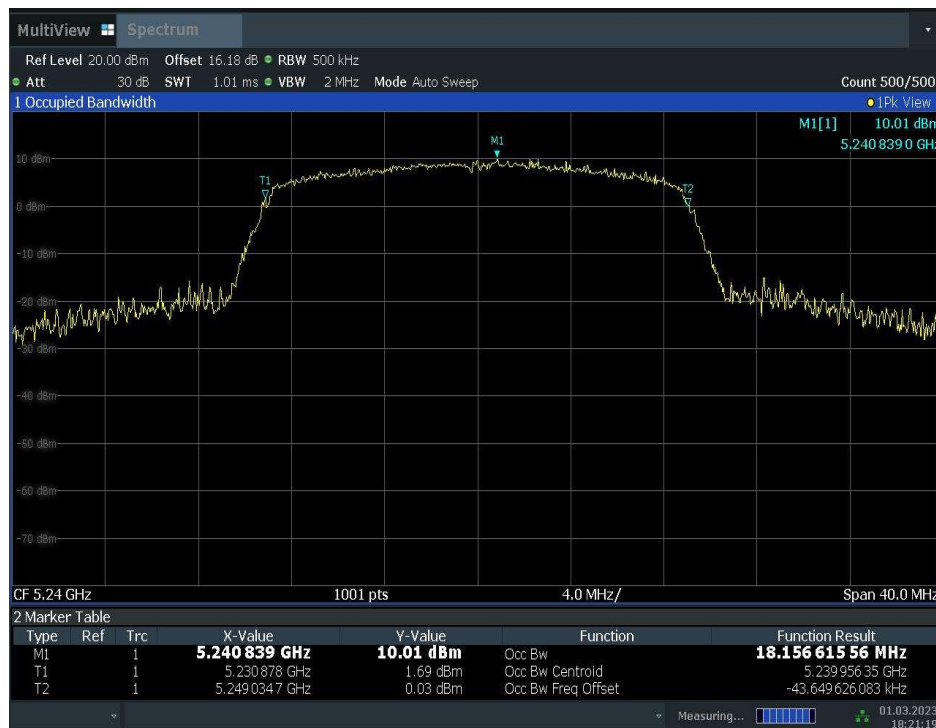
Fig.38 99% Occupied bandwidth (802.11n-HT20, 5240MHz)
