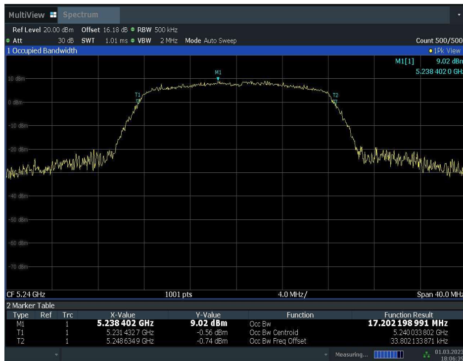
Fig.35 99% Occupied bandwidth (802.11a, 5240MHz)
