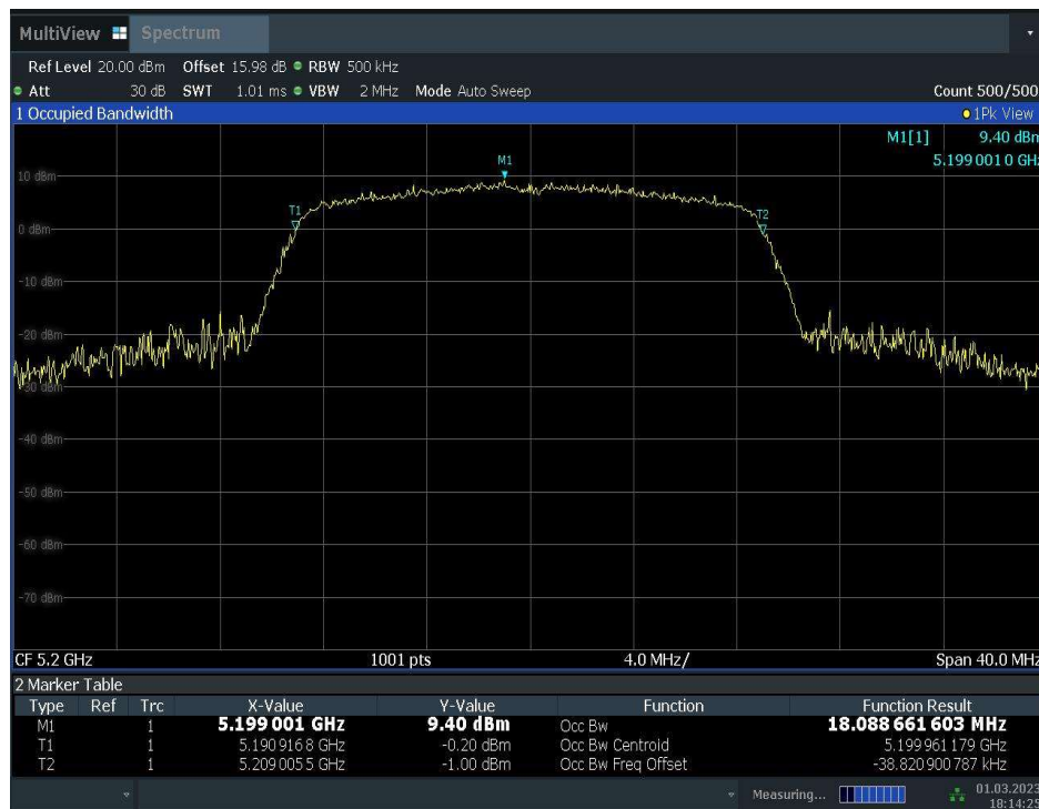
Fig.37 99% Occupied bandwidth (802.11n-HT20, 5200MHz)
