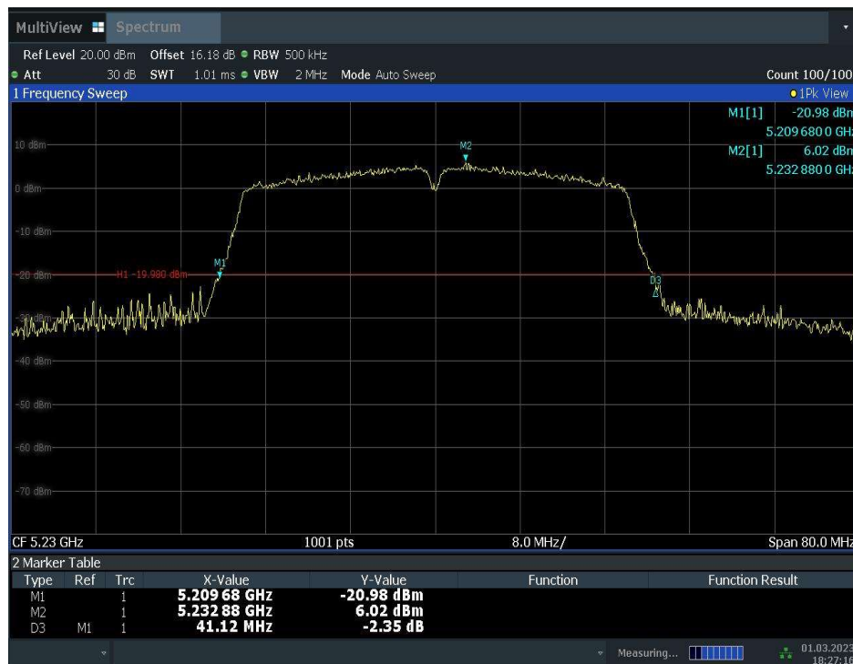
Fig.14 Occupied 26dB Bandwidth (802.11ac-HT40, 5230MHz)
