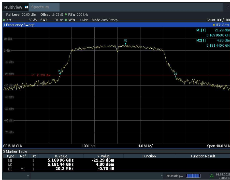
Fig.1 Occupied 26dB Bandwidth (802.11a, 5180MHz)
