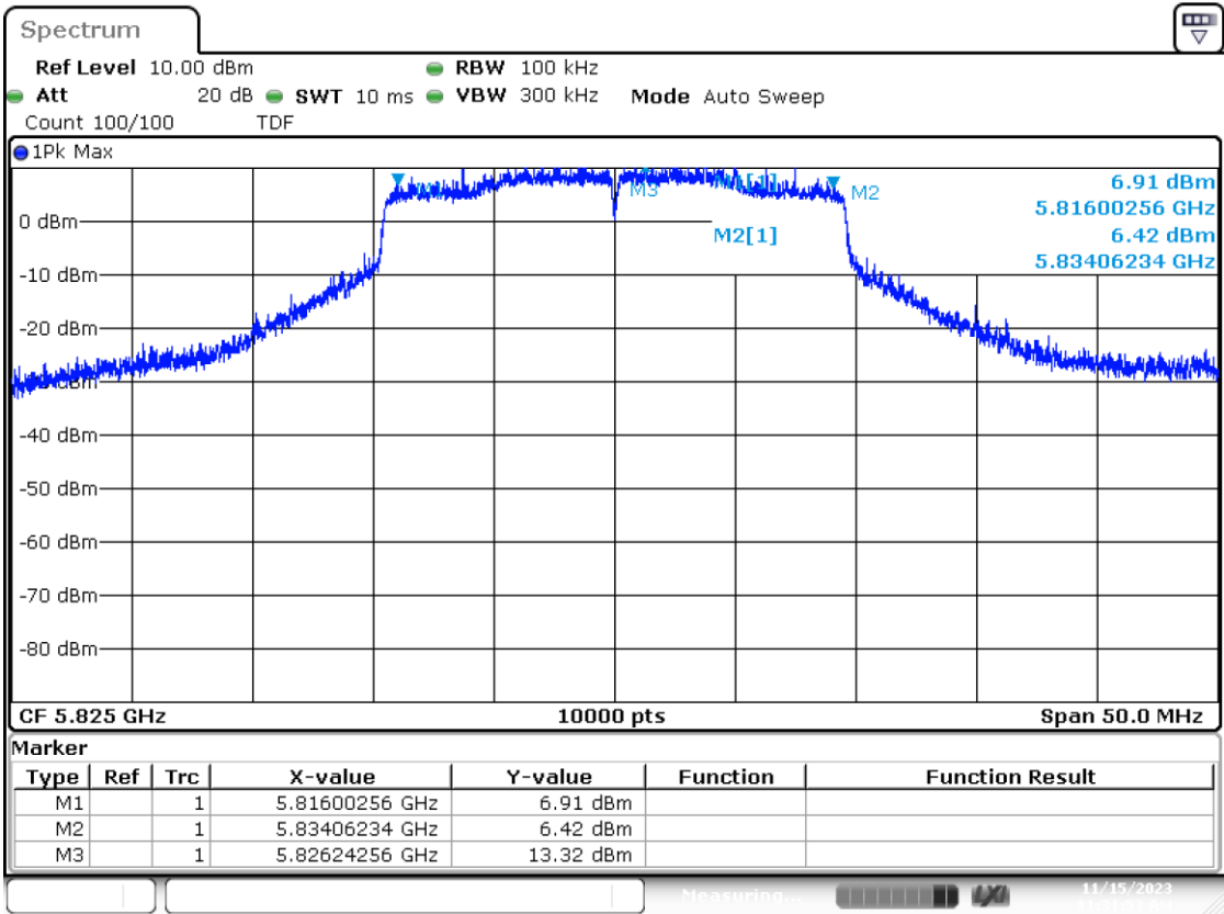
SISO A-802.11ax/be20-CH165-5825MHz-MCS0
