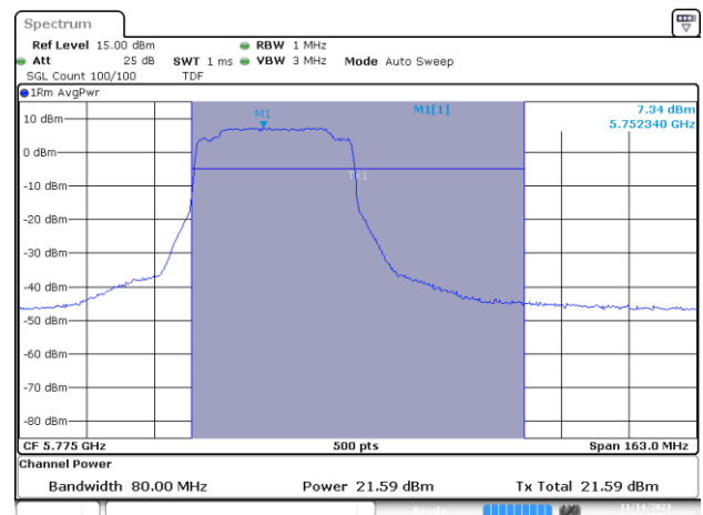
MIMO B-802.11ax/be80-CH155-5775MHz-MCS0 40m
