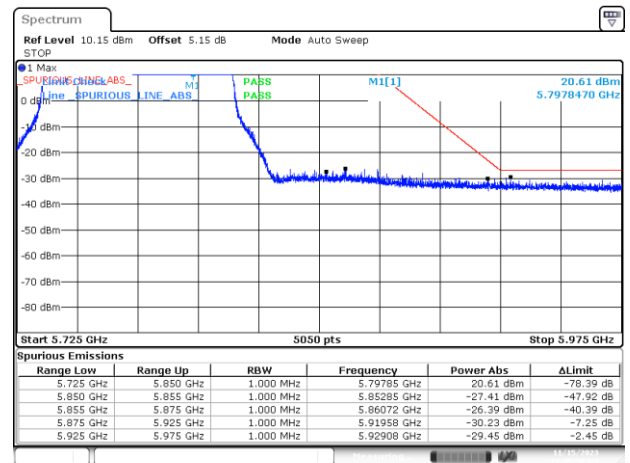
BE-NR-HIGH, SISO-A, 802.11ax/be80-MCS0, Ch155
