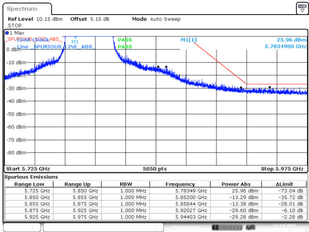
BE-NR-HIGH, SISO-B, 802.11ax/be40-MCS0, Ch159
