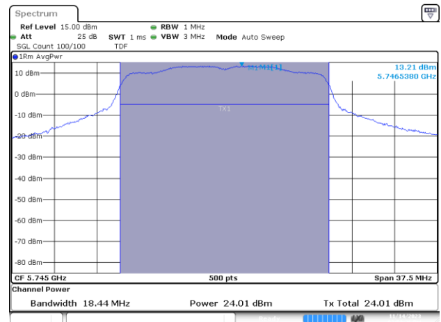
MIMO B-802.11n20-CH149-5745MHz-HT8 FullBW
