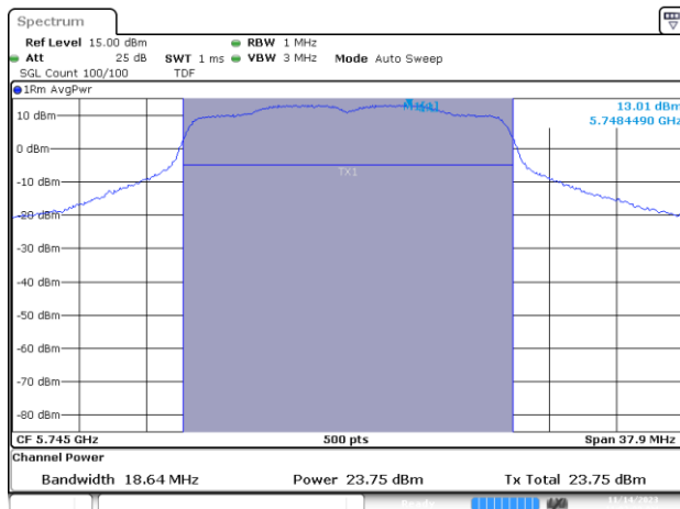
MIMO A-802.11n20-CH149-5745MHz-HT8 FullBW
