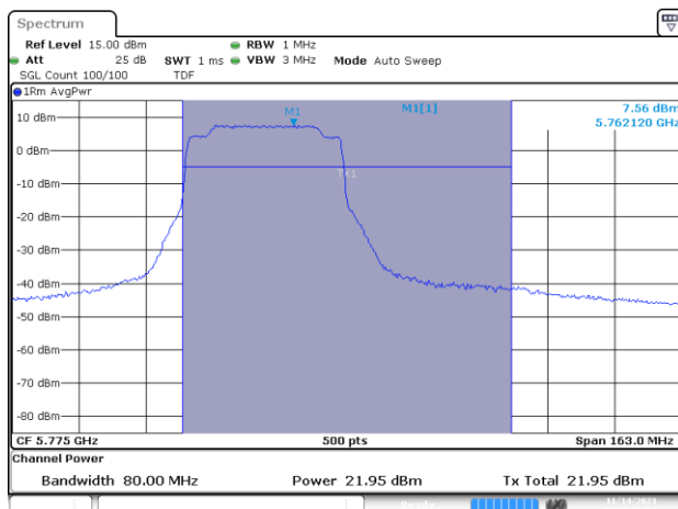
MIMO A-802.11ax/be80-CH155-5775MHz-MCS0 40m
