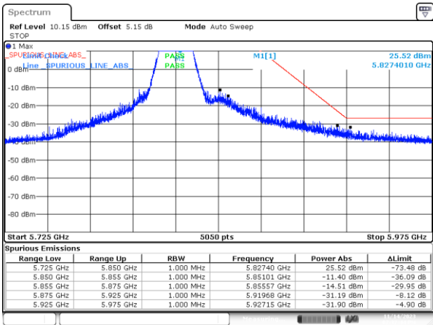
BE-NR-HIGH, MIMO-A, 802.11n20-HT0, Ch165
