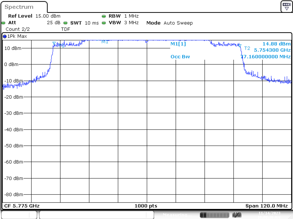
SISO B-802.11ax/be80-CH155-5775MHz-MCS0
