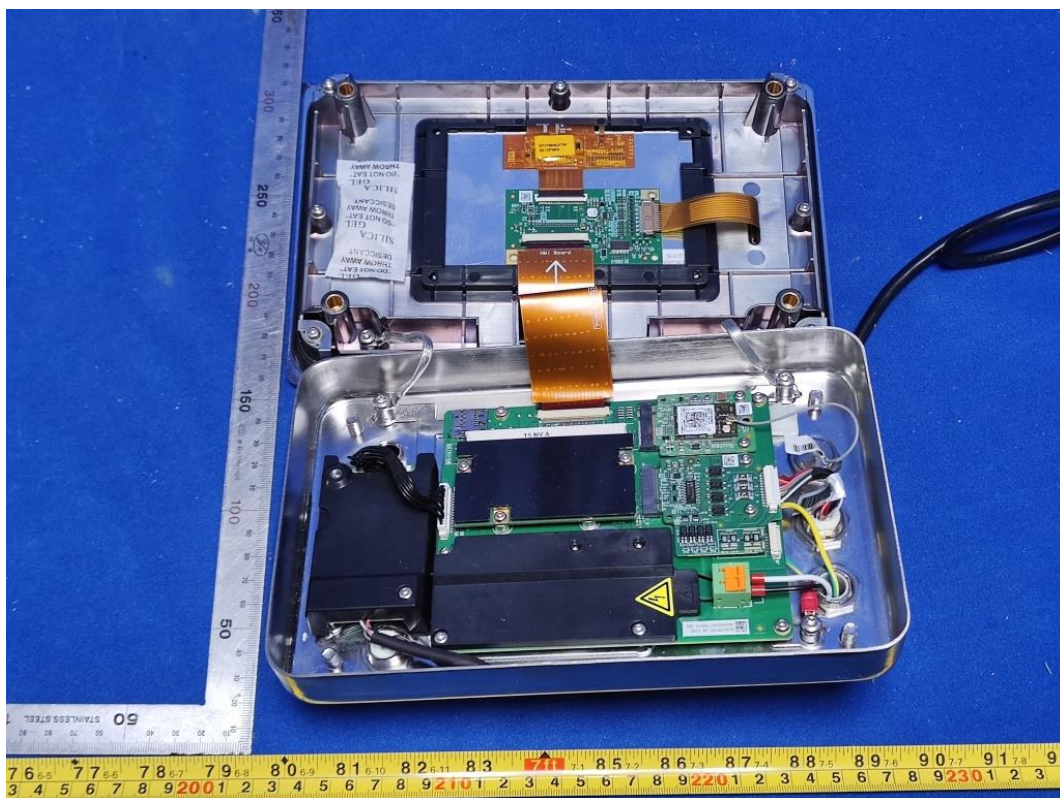
FIGURE 8 IND400 (IND400) COVER REMOVE2
