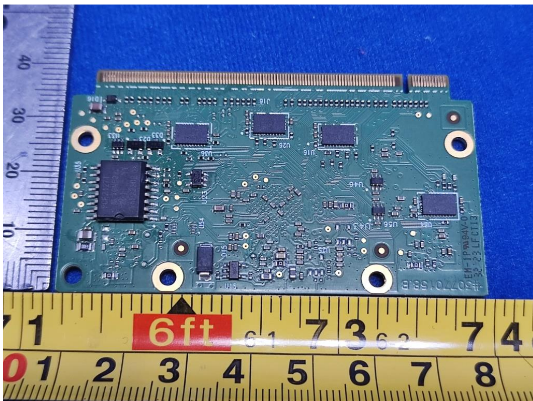
FIGURE 16 IND400 (IND400) MAIN BOARD2 BACK
