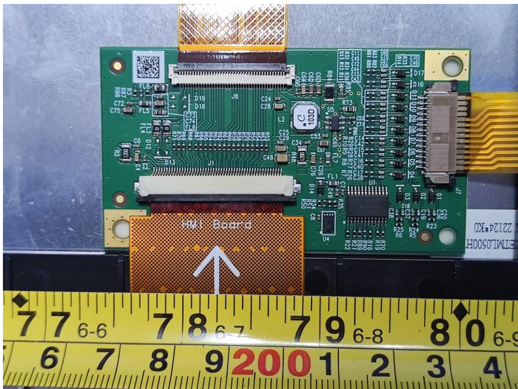
FIGURE 22 IND400 (IND400) PANEL BOARD
