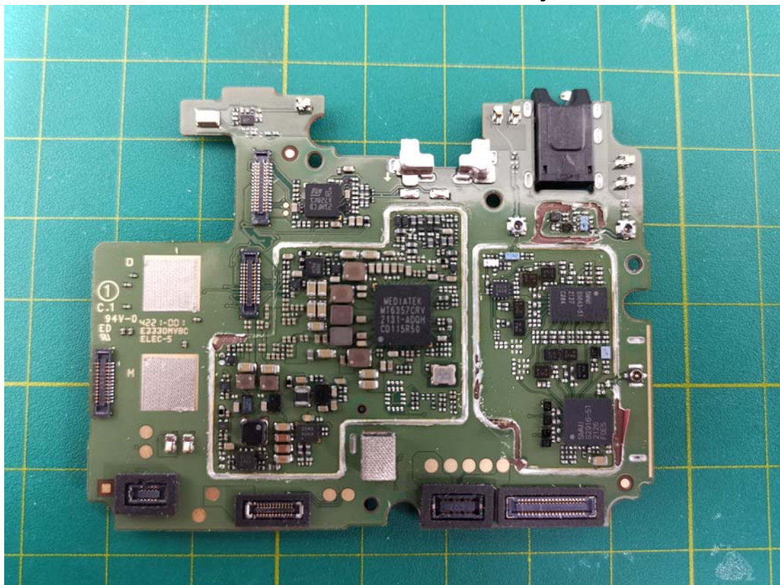
6102H Mobile Phone Disassembly
