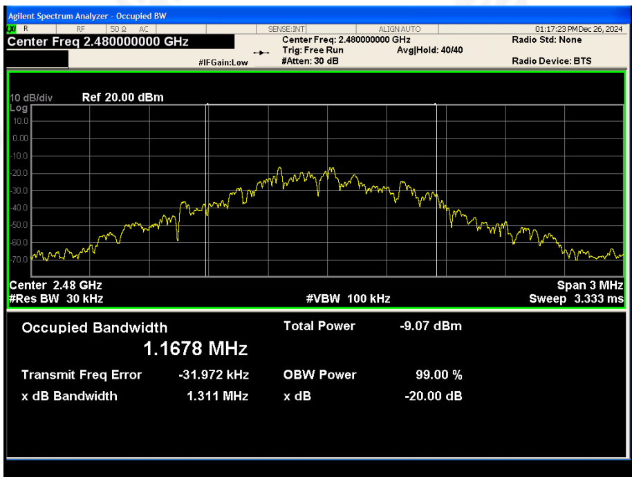
CH39: 2480MHz
