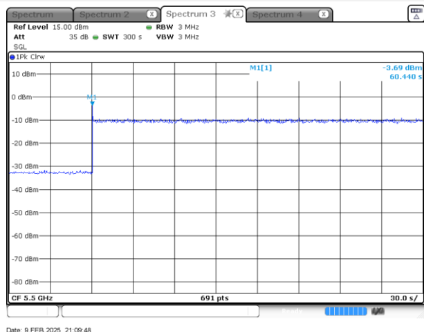
11a-5500 MHz
