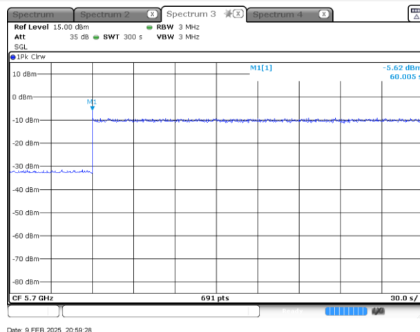
11a-5700 MHz
