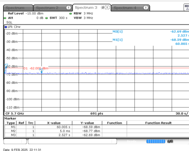
11a-5700 MHz
