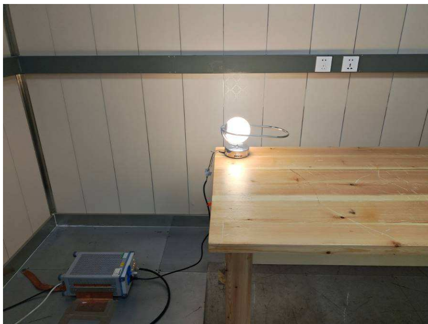
Conducted Disturbance
