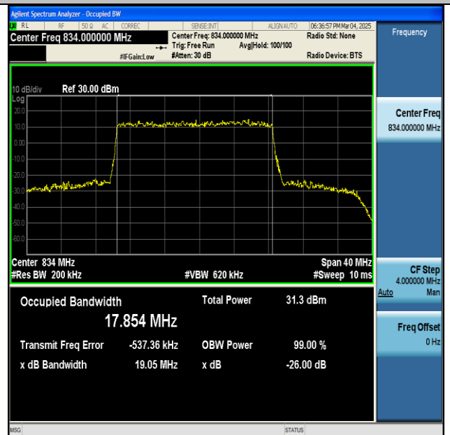
NTNV-n5-PC3-15-20-L-DFT-16QAM-Outer_Full-Ant1-PASS
