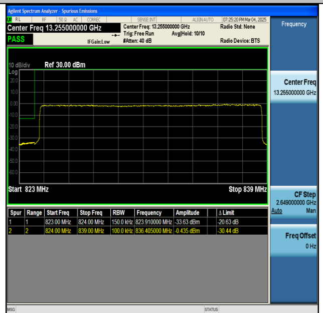
NTNV-n5-PC3-15-15-L-CP-QPSK-Outer_Full-PASS
