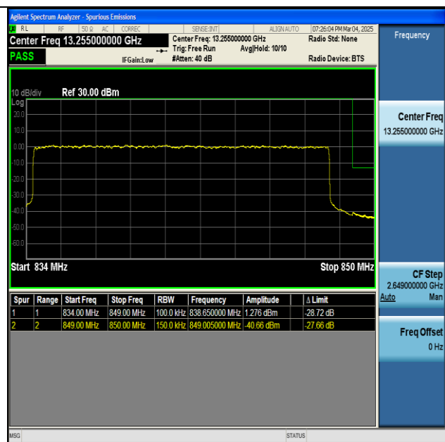
NTNV-n5-PC3-15-15-H-DFT-BPSK-Outer_Full-PASS
