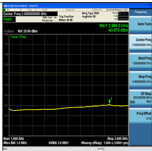
NTNV-n5-PC3-15-20-L-CP-QPSK-Edge_1RB_Left-1000-3000-PASS
