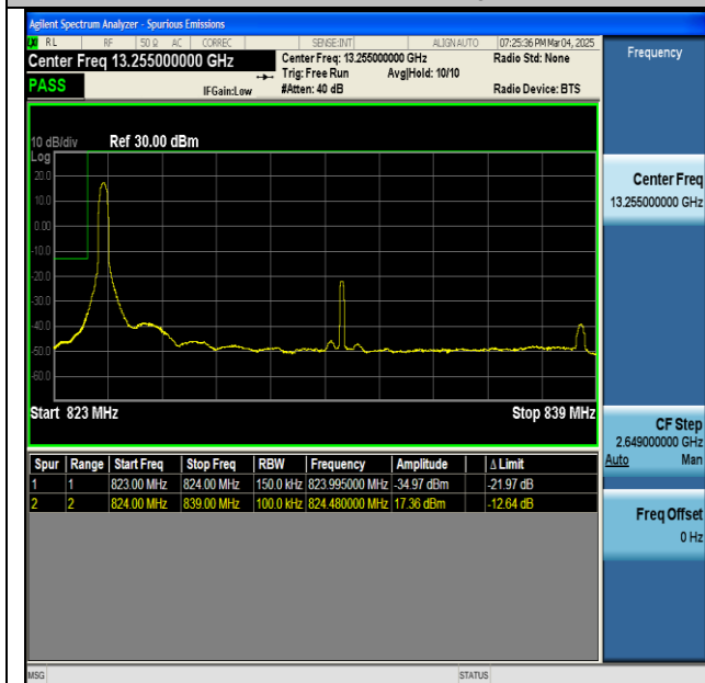
NTNV-n5-PC3-15-15-L-CP-QPSK-Edge_1RB_Left-PASS
