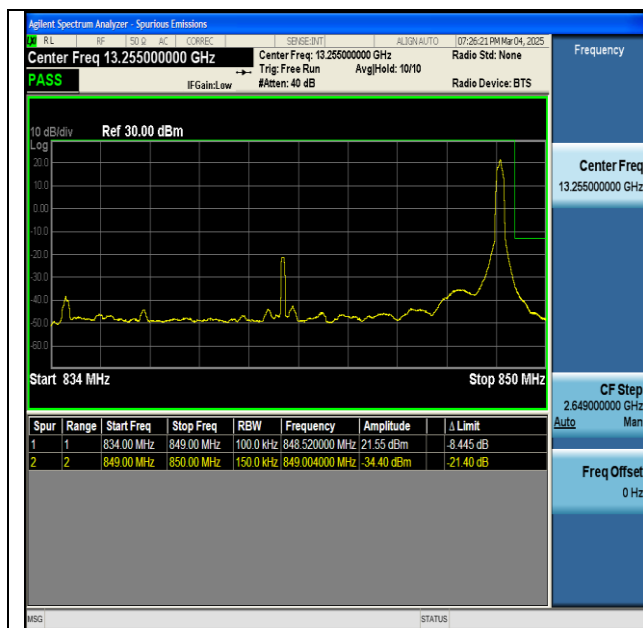
NTNV-n5-PC3-15-15-H-DFT-BPSK-Edge_1RB_Right-PASS
