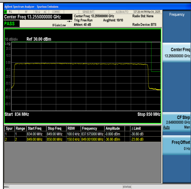
NTNV-n5-PC3-15-15-H-CP-QPSK-Outer_Full-PASS
