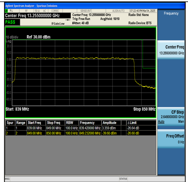
NTNV-n5-PC3-15-10-H-DFT-BPSK-Outer_Full-PASS
