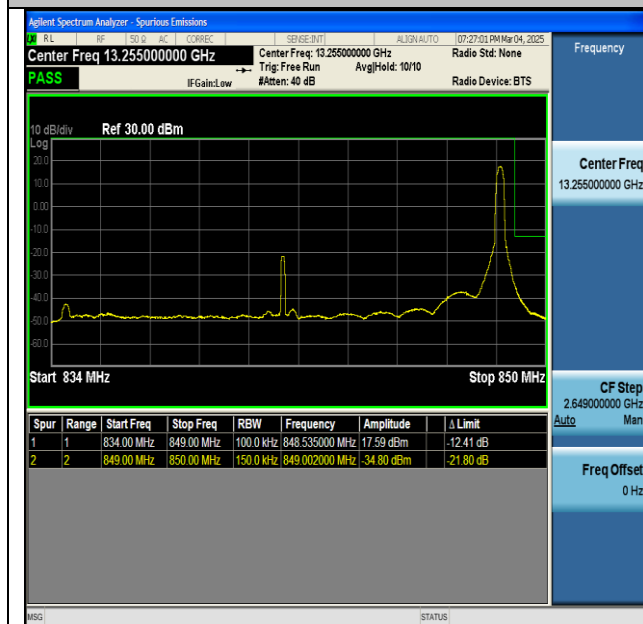
NTNV-n5-PC3-15-15-H-CP-QPSK-Edge_1RB_Right-PASS
