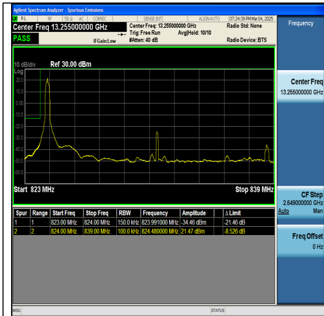
NTNV-n5-PC3-15-15-L-DFT-BPSK-Edge_1RB_Left-PASS
