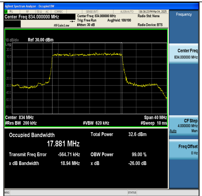
NTNV-n5-PC3-15-20-L-DFT-BPSK-Outer_Full-Ant1-PASS
