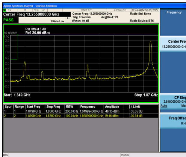
Band25_20MHz_QPSK_26140_1RB#99
