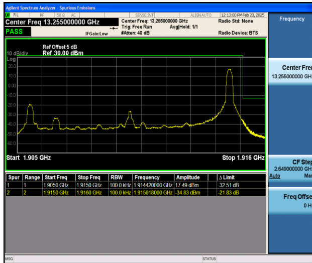
Band25_10MHz_16QAM_26640_1RB#49
