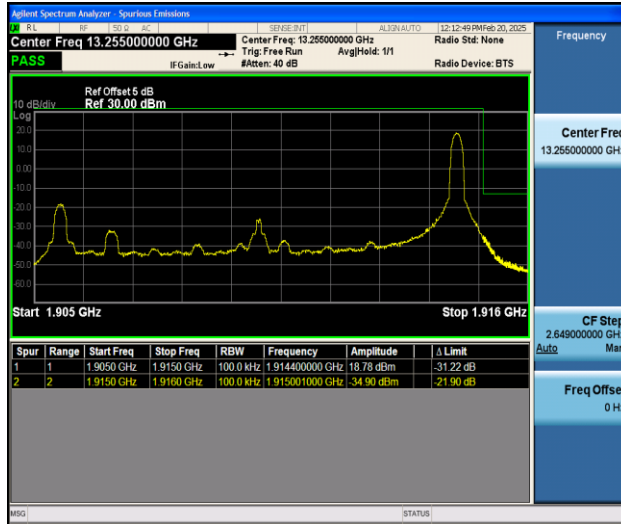
Band25_10MHz_QPSK_26640_1RB#49
