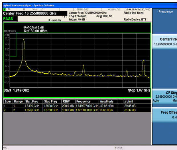
Band25_20MHz_16QAM_26140_1RB#0
