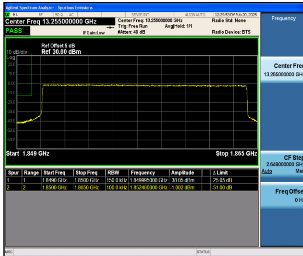
Band25_15MHz_QPSK_26115_75RB#0
