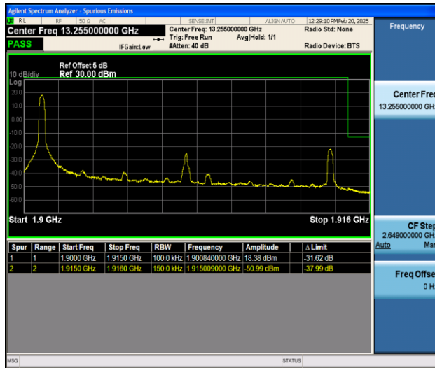
Band25_15MHz_16QAM_26615_1RB#0
