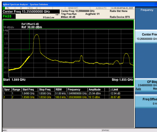
Band25_5MHz_16QAM_26065_1RB#0
