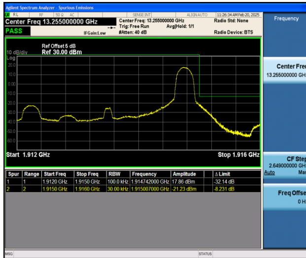
Band25_3MHz_16QAM_26675_1RB#14
