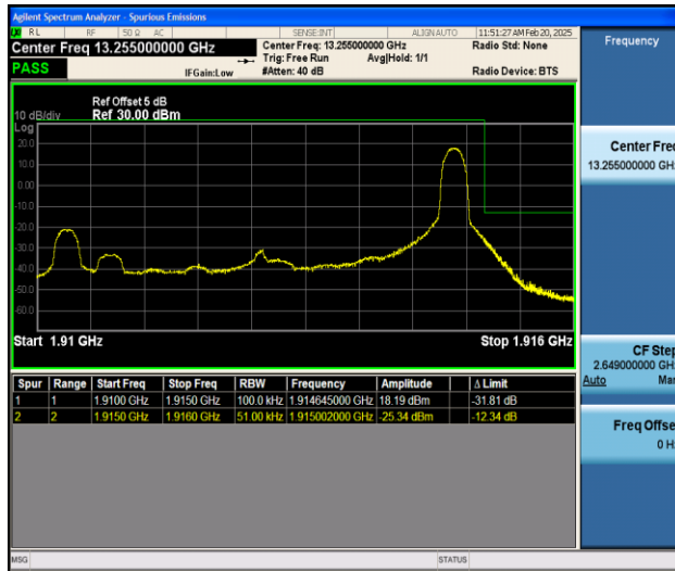
Band25_5MHz_16QAM_26665_1RB#24
