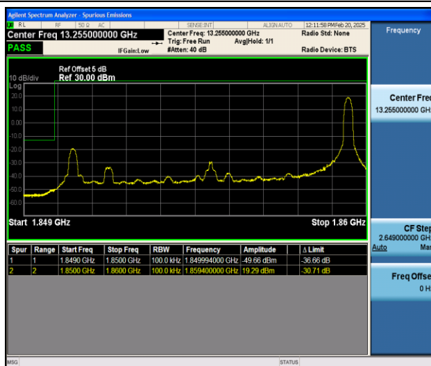
Band25_10MHz_QPSK_26090_1RB#49
