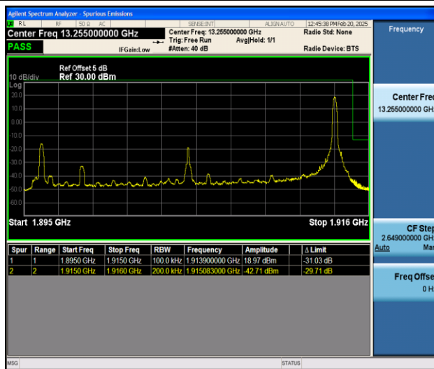
Band25_20MHz_QPSK_26590_1RB#99
