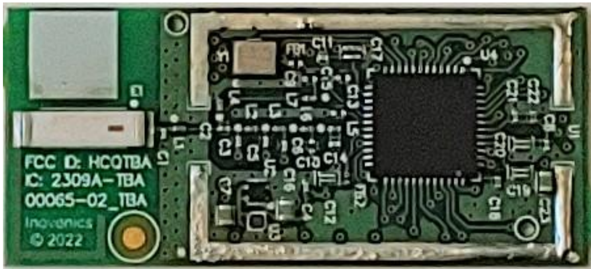
TBA Silkscreen Label - Top
