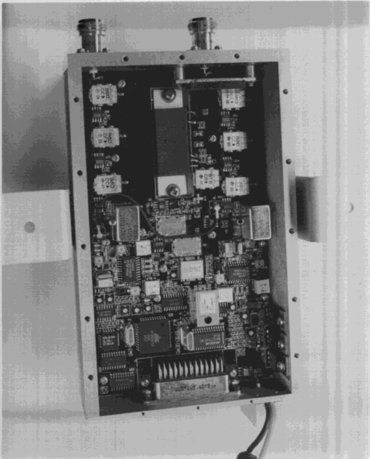
6.6 Photo: EUT with cover removed
