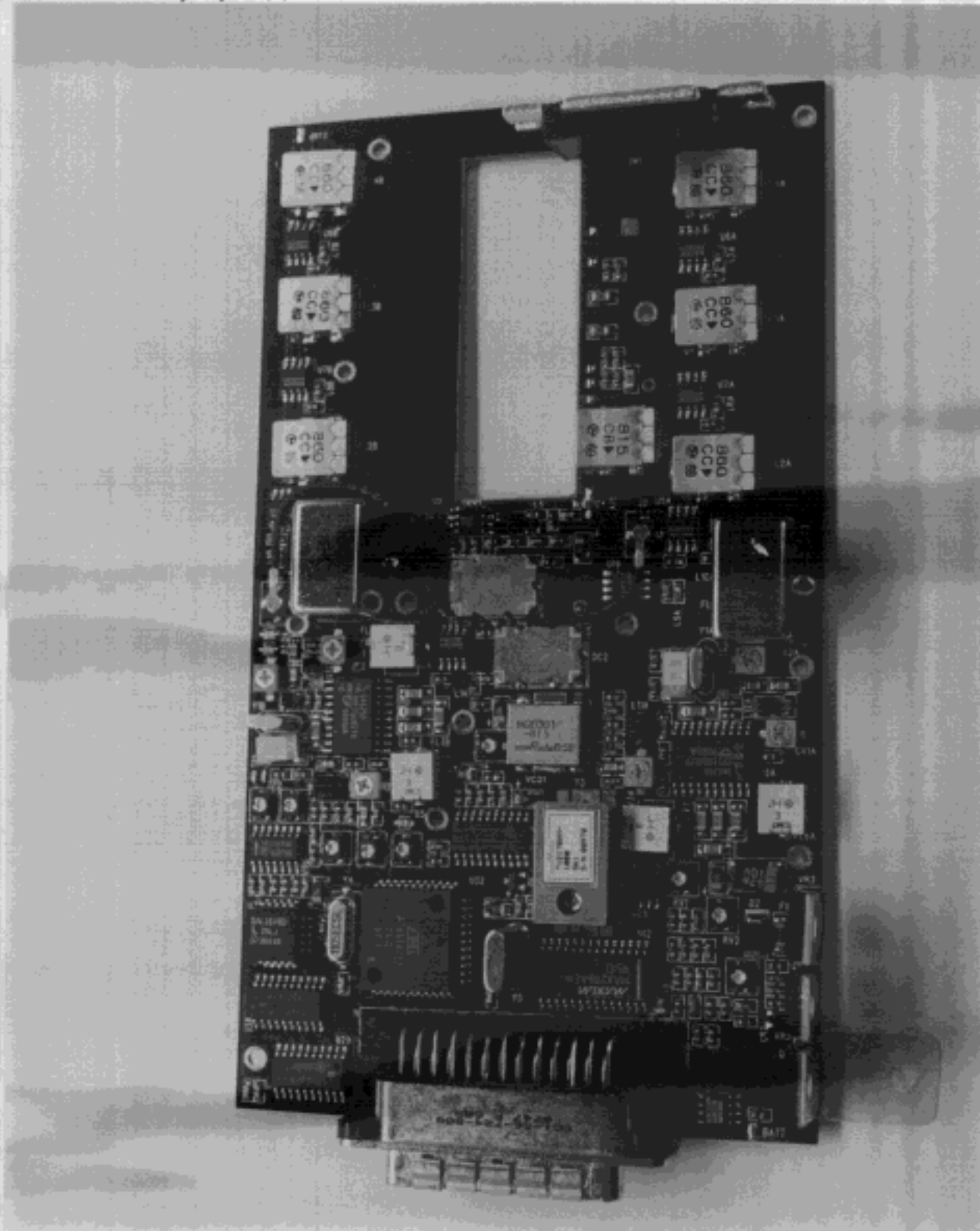
6.7 Photo: EUT PCB Circuitry Layout (1)
