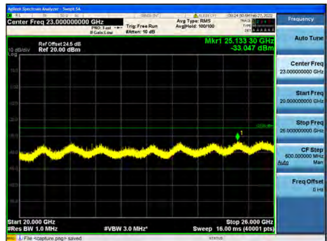
Band7-20G-26G / 5MHz / High CH / 64QAM
