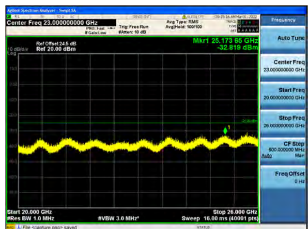
Band7-20G-26G / 10MHz / Low CH / 64QAM
