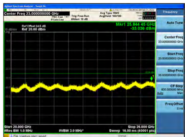
Band7-20G-26G / 5MHz / Low CH / 64QAM
