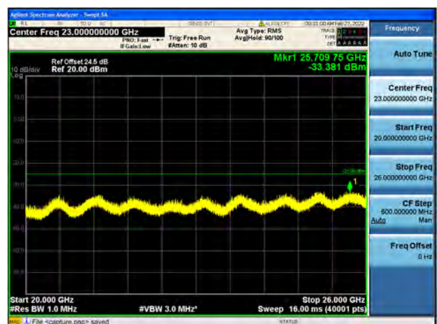
Band7-20G-26G / 10MHz / Mid CH / 64QAM
