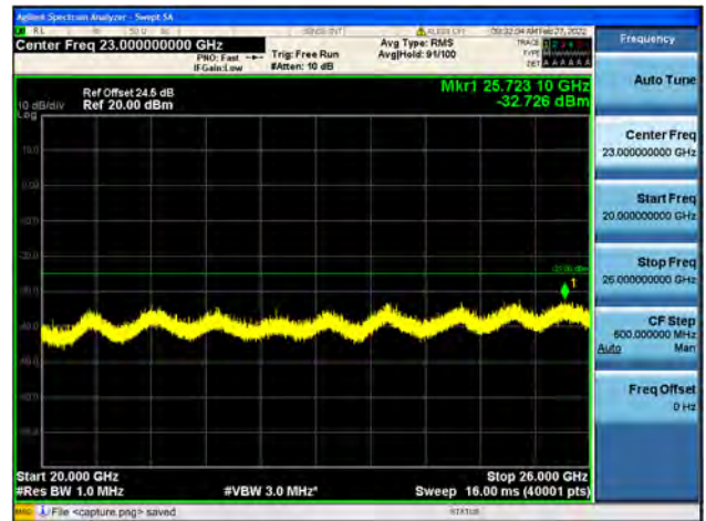
Band7-20G-26G / 10MHz / High CH / 16QAM
