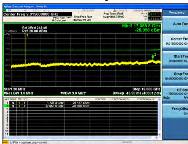
Band4 / 20MHz / High CH / 64QAM
