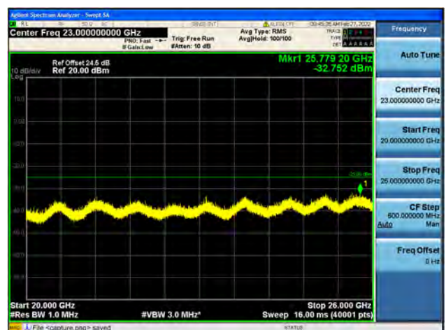
Band7-20G-26G / 20MHz / Low CH / 64QAM
