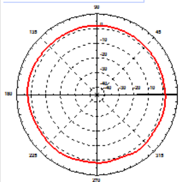
H-Plane Radiation Pattern
