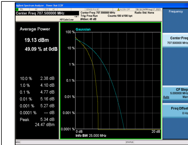
Band12-3MHz-QPSK-23095-15RB#0-PASS
