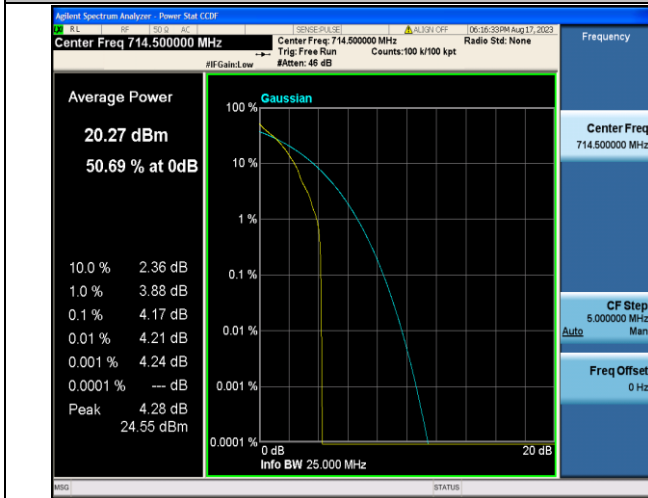
Band12-3MHz-QPSK-23165-1RB#0-PASS
