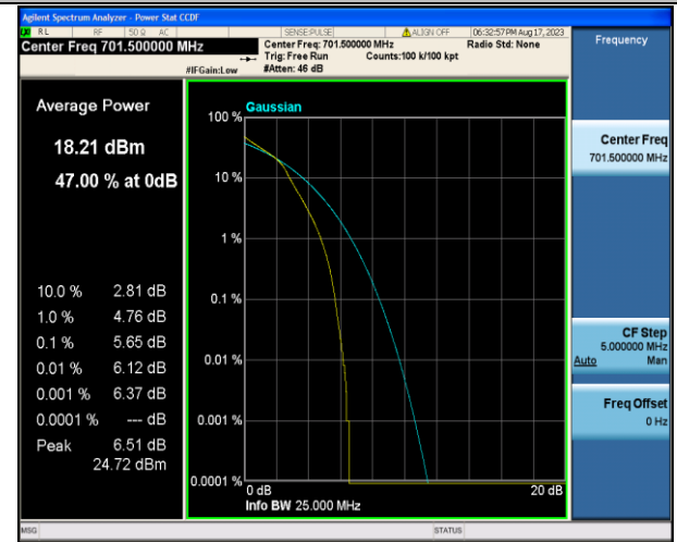
Band12-5MHz-16QAM-23035-25RB#0-PASS
