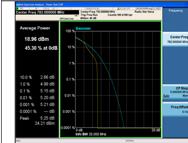
Band13-5MHz-16QAM-23230-1RB#0-PASS
