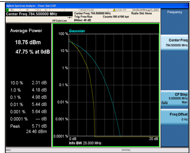
Band13-5MHz-QPSK-23255-25RB#0-PASS
