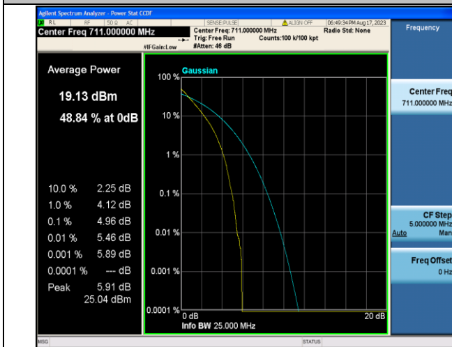
Band12-10MHz-QPSK-23130-50RB#0-PASS
