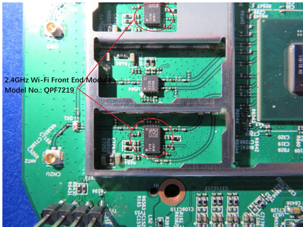
(14) EUT Photo (2.4GHz Wi-Fi Front End Module, Model No.: QPF7219)
