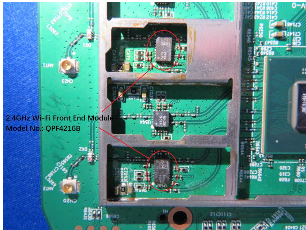
(1) EUT Photo (2.4GHz Wi-Fi Front End Module, Model No.: QPF4216B)
