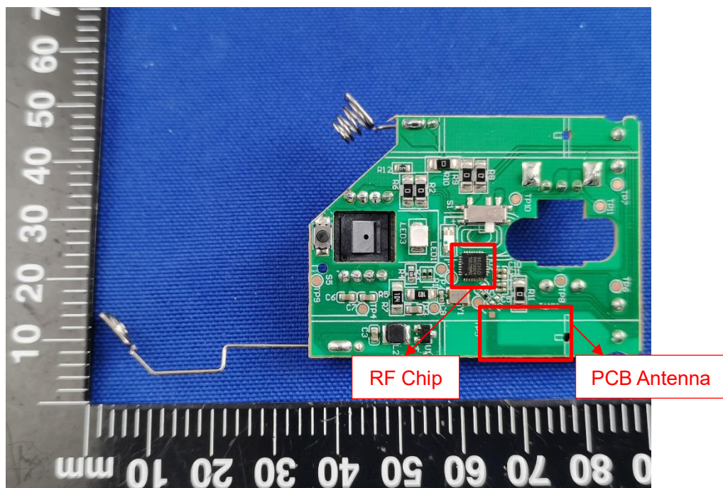
MAIN BOARD REAR VIEW
