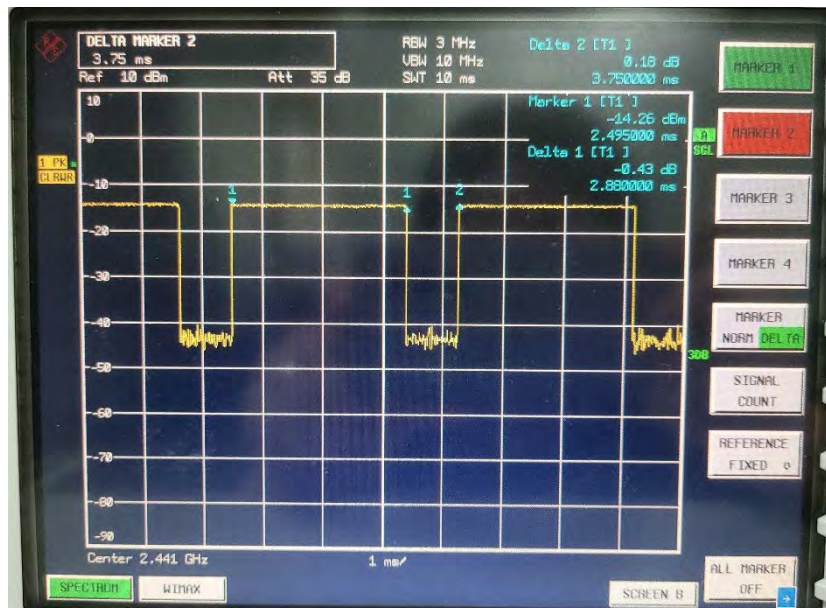
Figure 8.2 Bluetooth Transmission Plot
