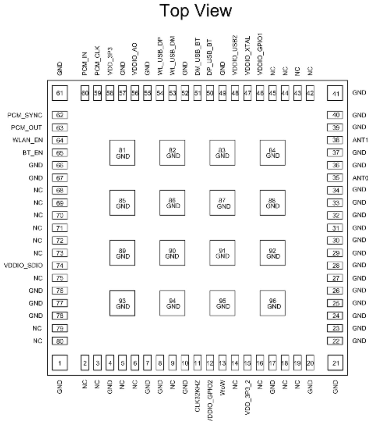
Figure 2: BALI Module Pin Diagram
