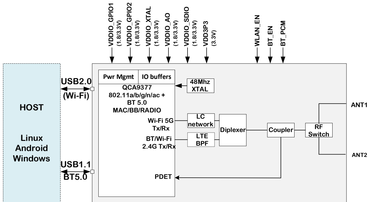
Figure 1: BALI Block Diagram with Antenna Pin
