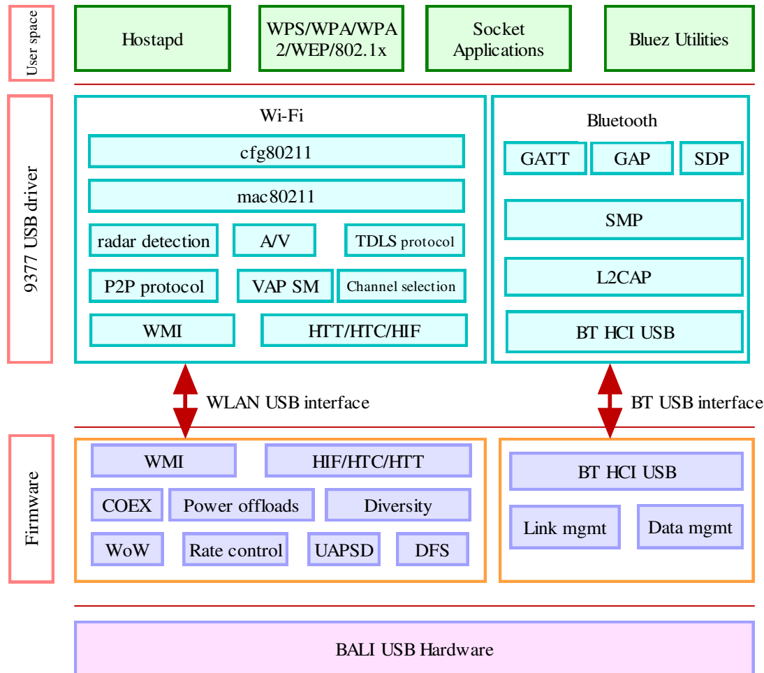
Figure 3: BALI Software Block Diagram
