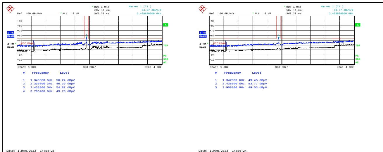
1000-4000MHz, WiFi ch06 11g 6M Ant0 + GSM1900 ch725 VP
