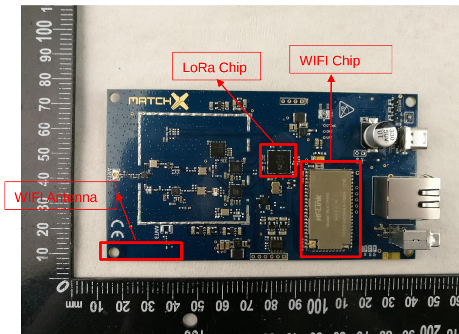
MAIN BOARD 1 FRONT VIEW 1
