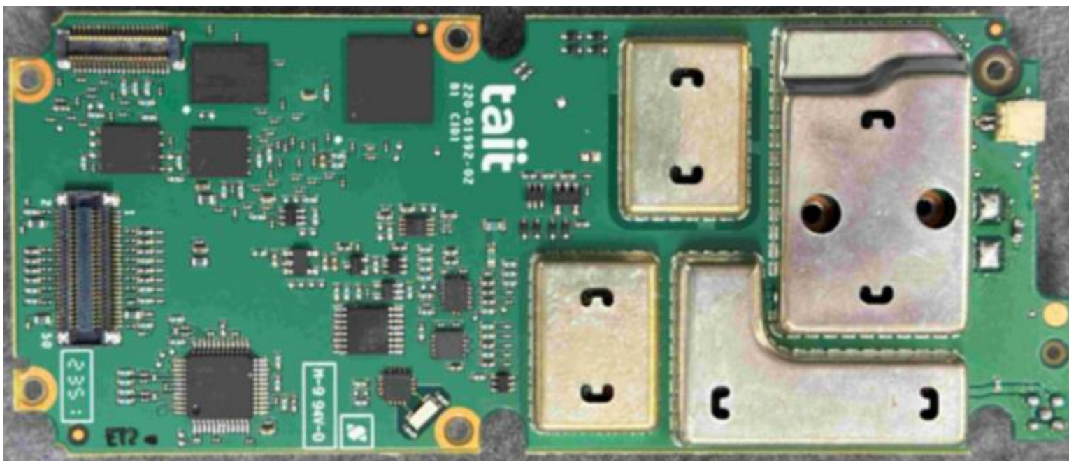
Photograph 01: Receive-Transmit PCB – top (with shields)
