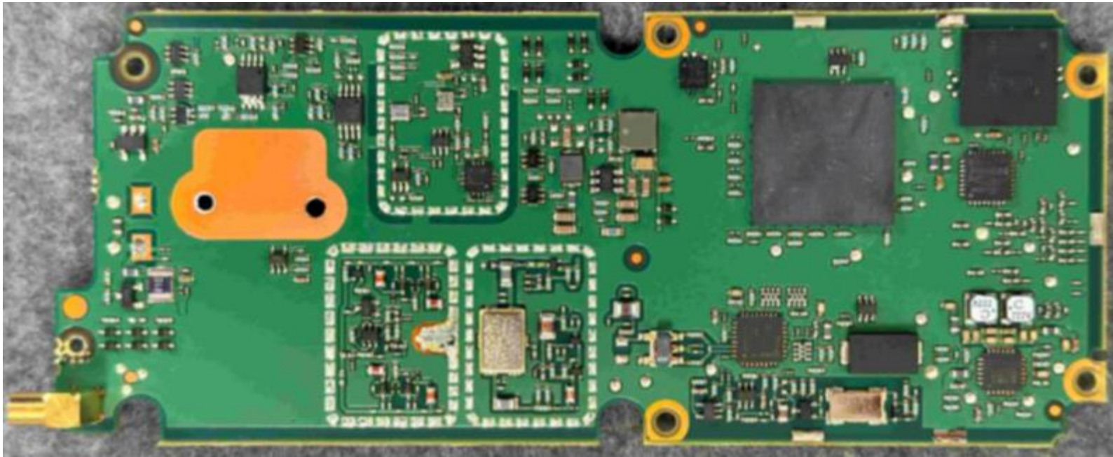
Photograph 04: Receive-Transmit PCB - bottom (without shields)
