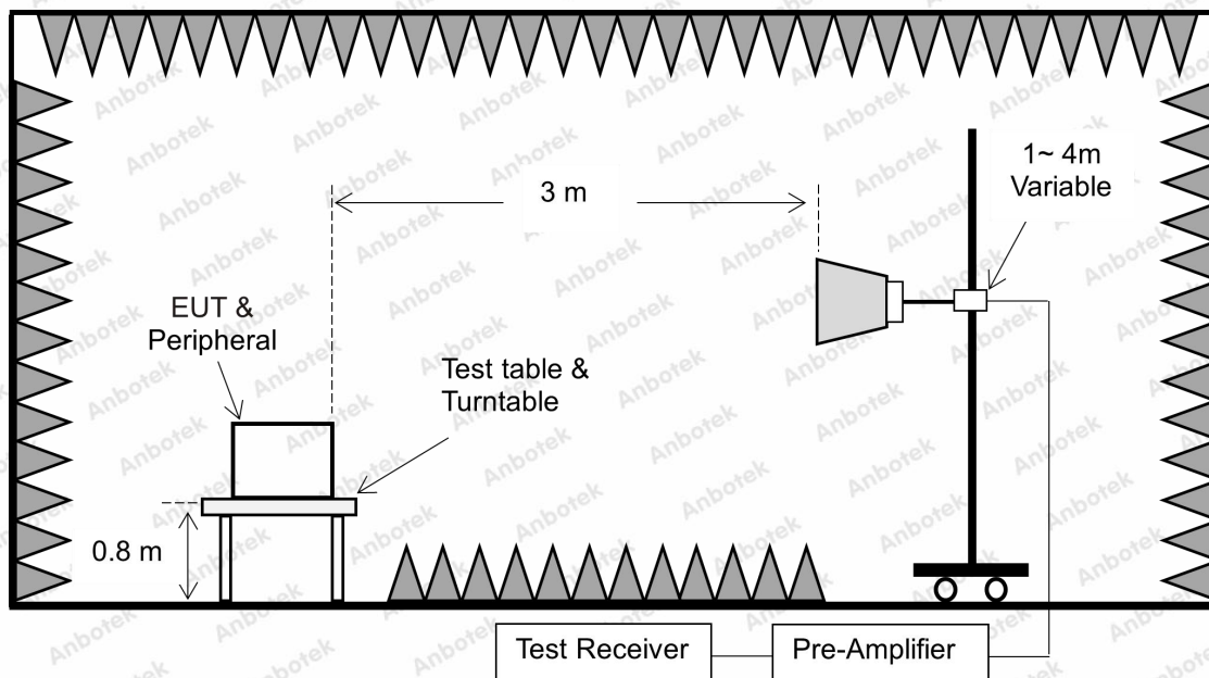
Figure 3. Above 1 GHz
