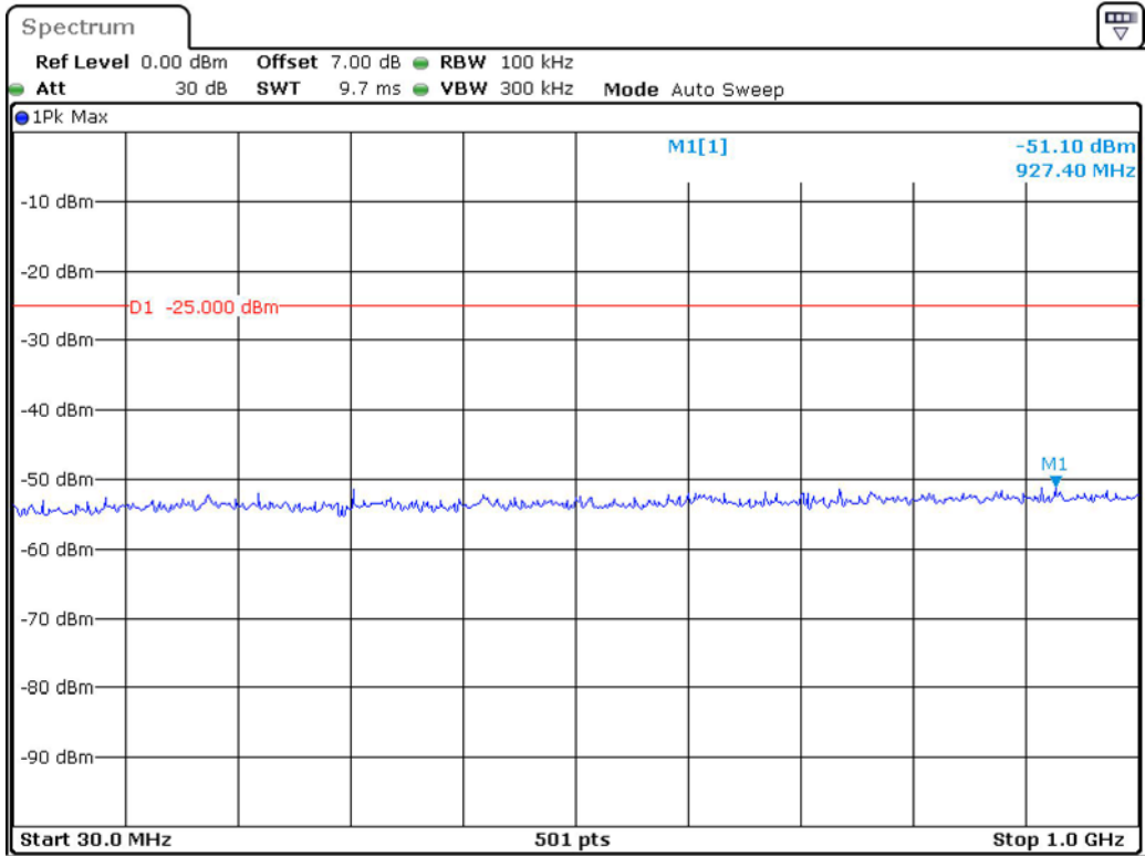
Band 41_15 MHz_High_QPSK_RB75#0_1(30MHz-1GHz)
