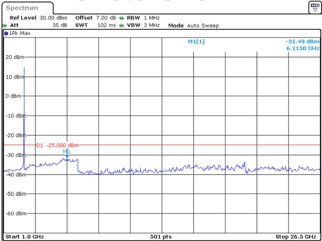
Band 41_15 MHz_High_QPSK_RB75#0_2(1GHz-26.5GHz)
