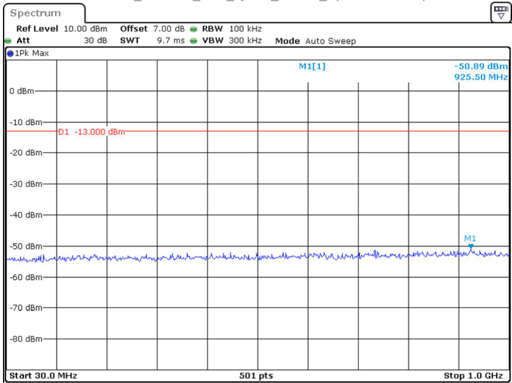
Band 66_1.4 MHz_Low_QPSK_RB6#0_1(30MHz-1GHz)
