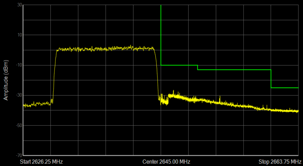
Band41 16QAM BW=15MHz Channel=41065 RB Size=75 Position=#0
