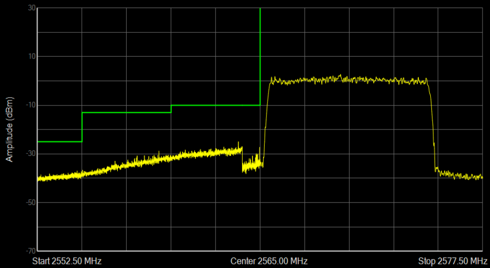
Band41 16QAM BW=10MHz Channel=40390 RB Size=50 Position=#0
