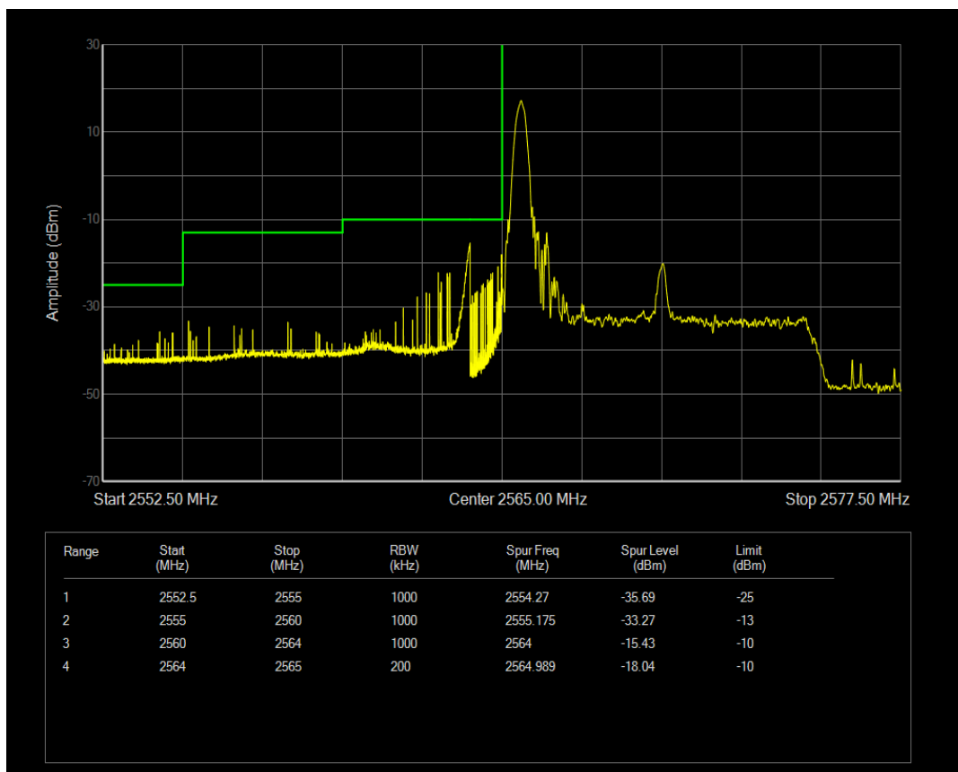
Band41 16QAM BW=10MHz Channel=40390 RB Size=1 Position=#Max
