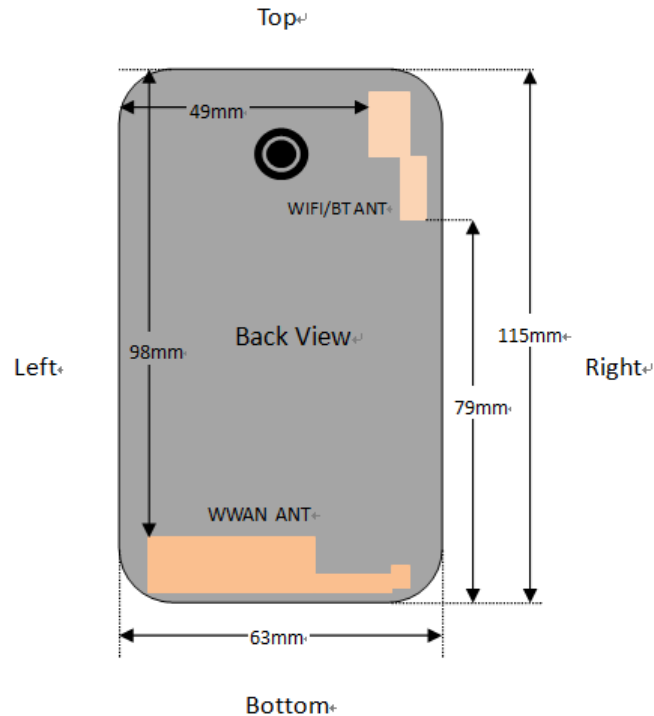
Fig.14.1 EUT Antenna Locations
