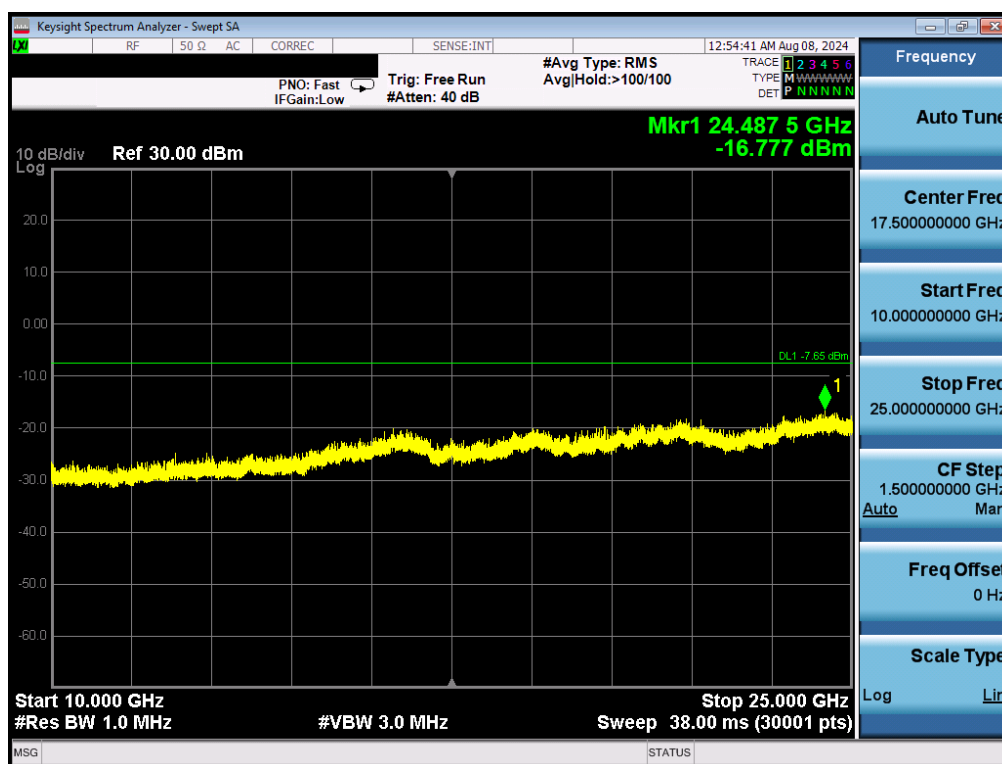
Plot 7-28. Conducted Spurious Plot (Bluetooth, GFSK, iPA – Ch. 78)
