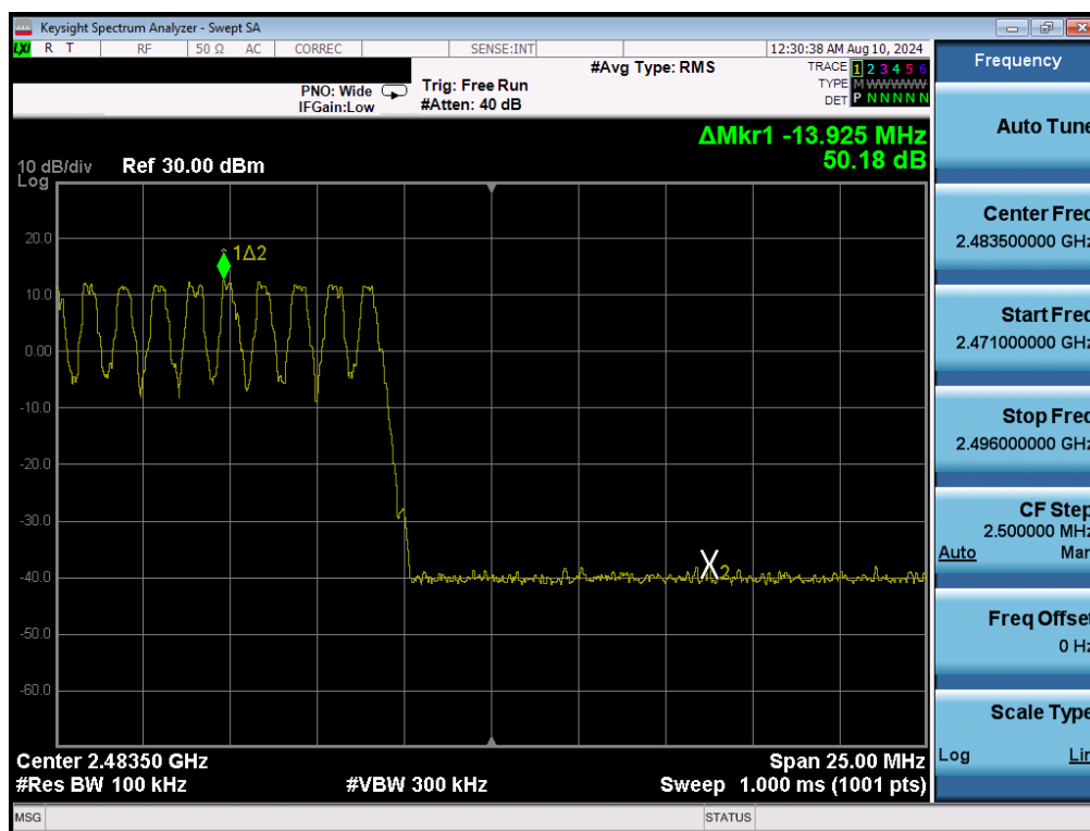
Plot 7-10. Band Edge Plot (Bluetooth with Hopping Enabled, GFSK, iPA)
