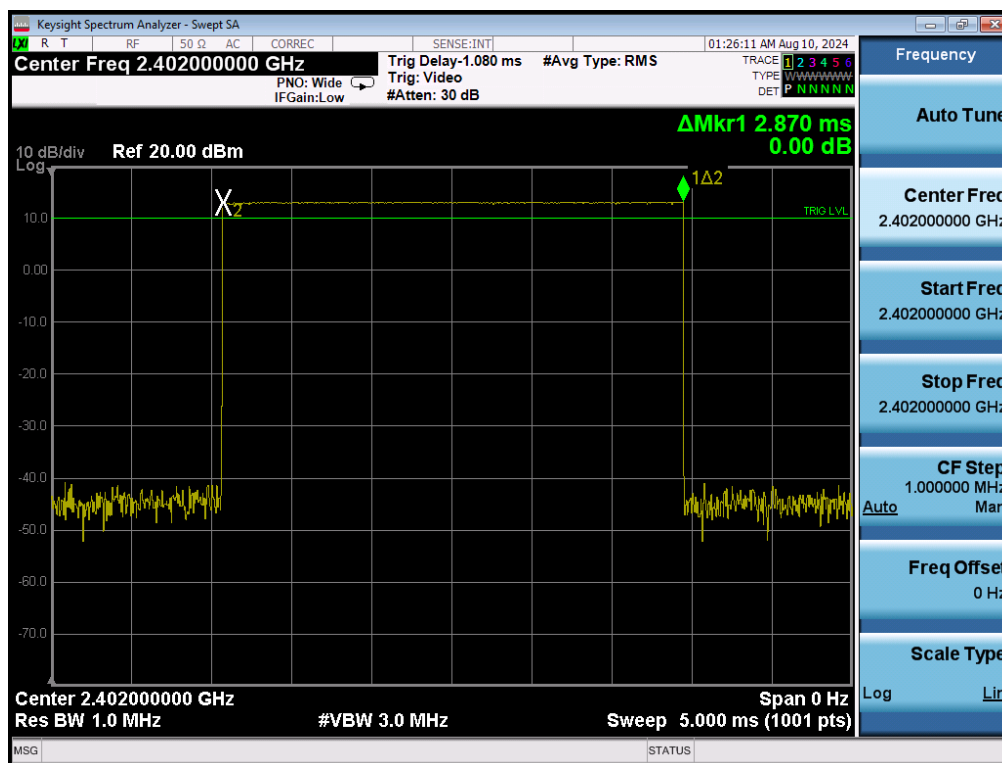
Plot 7-17. Time of Occupancy Plot (Bluetooth, GFSK, iPA)
