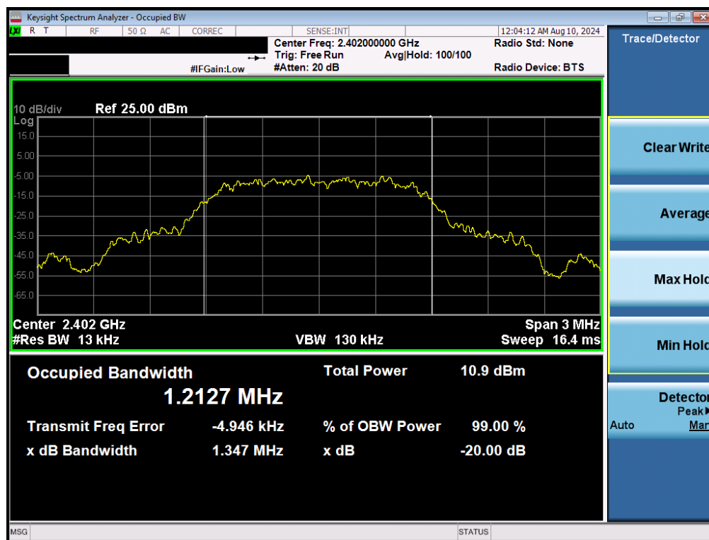
Plot 7-4. 20dB BW and 99% OBW Plot (Bluetooth, 8DPSK, iPA – Ch. 0)
