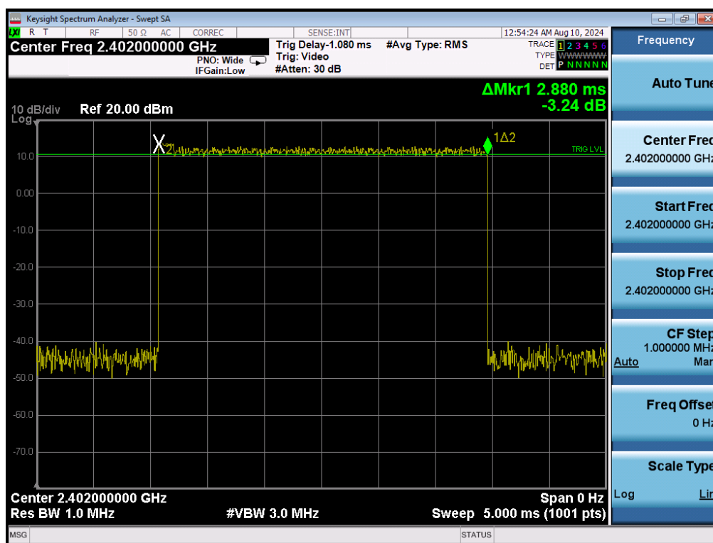
Plot 7-18. Time of Occupancy Plot (Bluetooth, 8DPSK, iPA)
