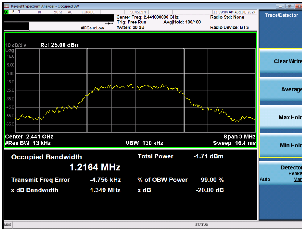
Plot 7-5. 20dB BW and 99% OBW Plot (Bluetooth, 8DPSK, iPA – Ch. 39)
