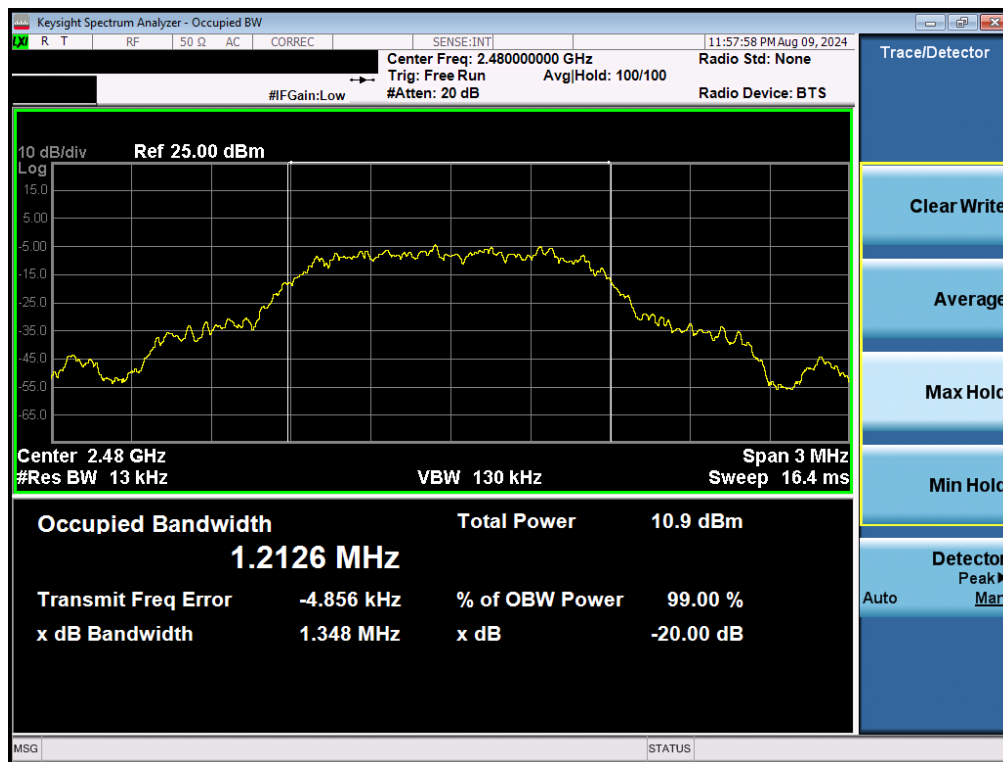
Plot 7-6. 20dB BW and 99% OBW Plot (Bluetooth, 8DPSK, iPA – Ch. 78)
