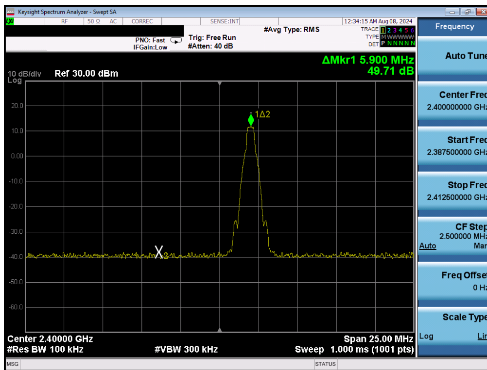
Plot 7-7. Band Edge Plot (Bluetooth with Hopping Disabled, GFSK, iPA – Ch. 0)
