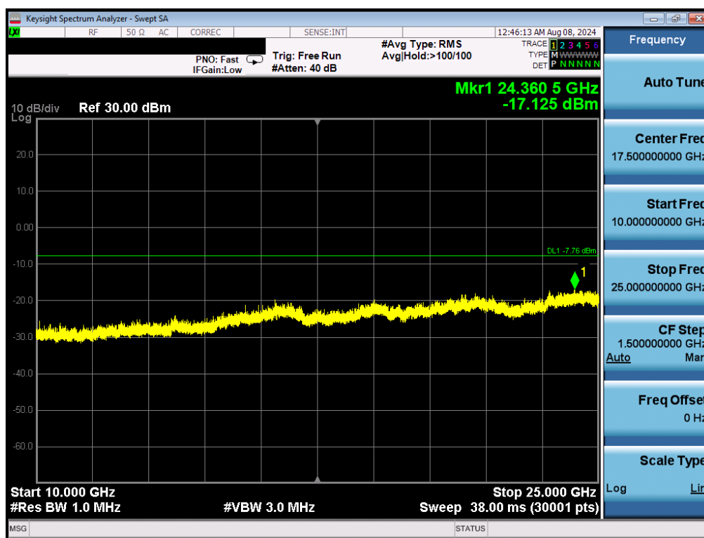
Plot 7-26. Conducted Spurious Plot (Bluetooth, GFSK, iPA - Ch. 39)
