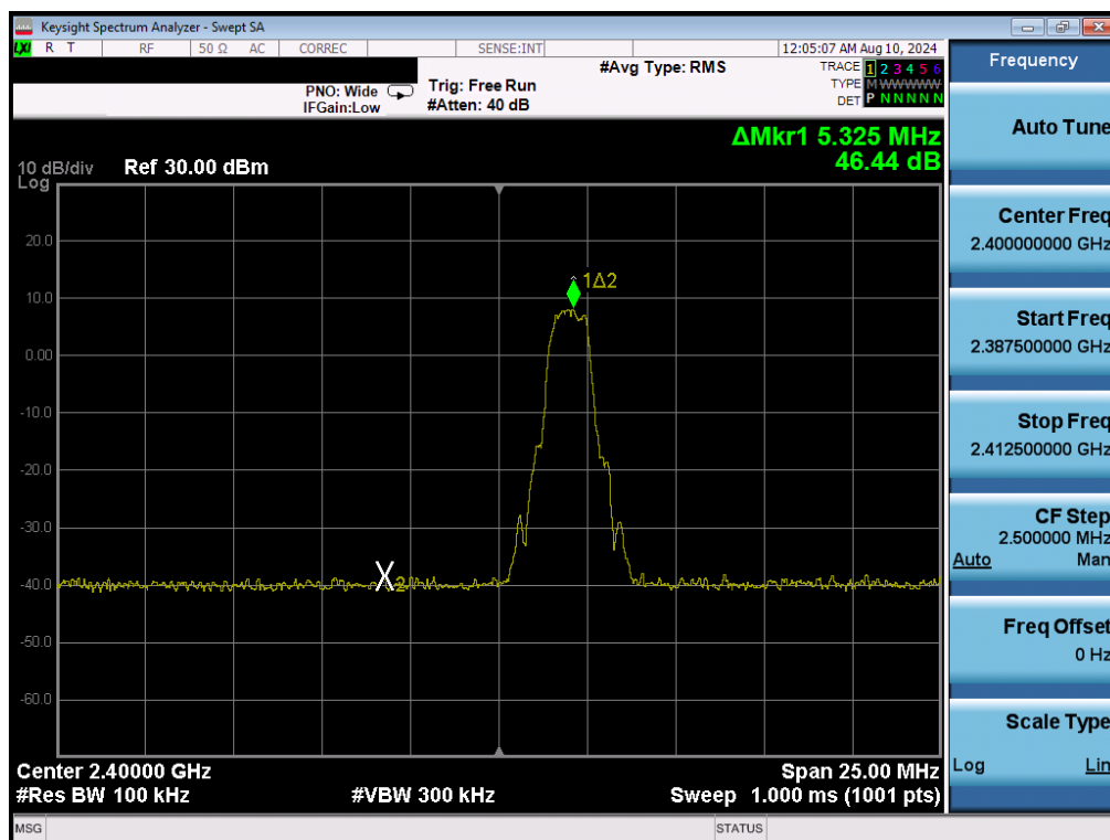
Plot 7-11. Band Edge Plot (Bluetooth with Hopping Disabled, 8DPSK, iPA – Ch. 0)
