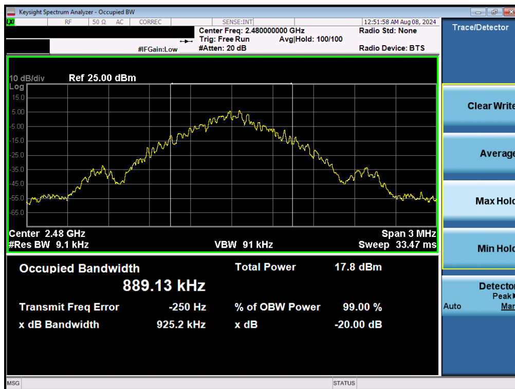
Plot 7-3. 20dB BW and 99% OBW Plot (Bluetooth, GFSK, iPA – Ch. 78)
