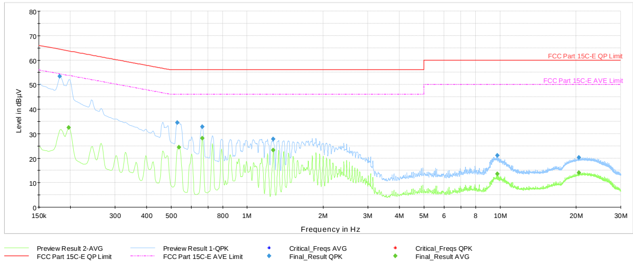
Plot 7-39. AC Line-Conducted Test Plot (N, GFSK, iPA – Ch.78, with host PC via USB-C cable with wire charger)
