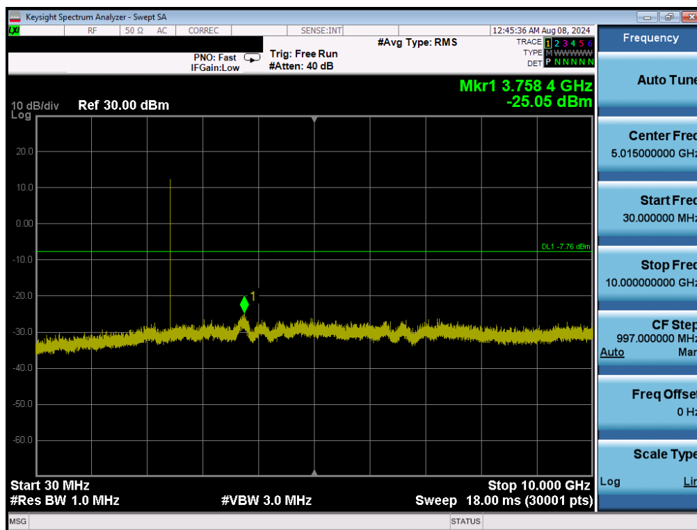
Plot 7-25. Conducted Spurious Plot (Bluetooth, GFSK, iPA – Ch. 39)
