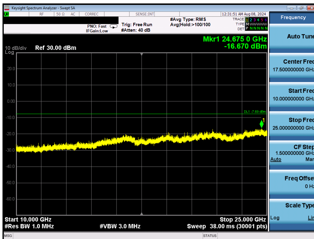
Plot 7-24. Conducted Spurious Plot (Bluetooth, GFSK, iPA – Ch. 0)
