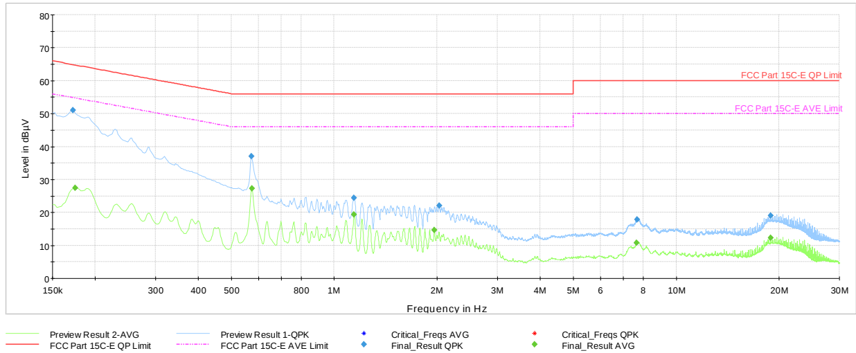
Plot 7-38. AC Line-Conducted Test Plot (L1, GFSK, iPA – Ch.78, with host PC via USB-C cable with wire charger)
