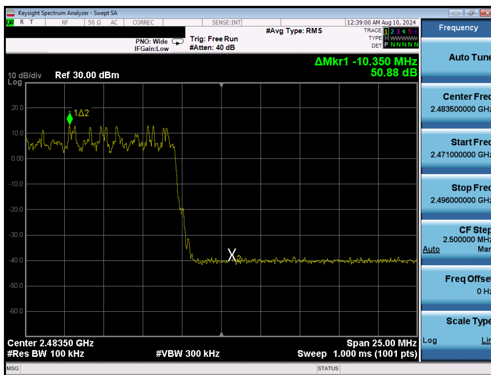
Plot 7-14. Band Edge Plot (Bluetooth with Hopping Enabled, 8DPSK, iPA)
