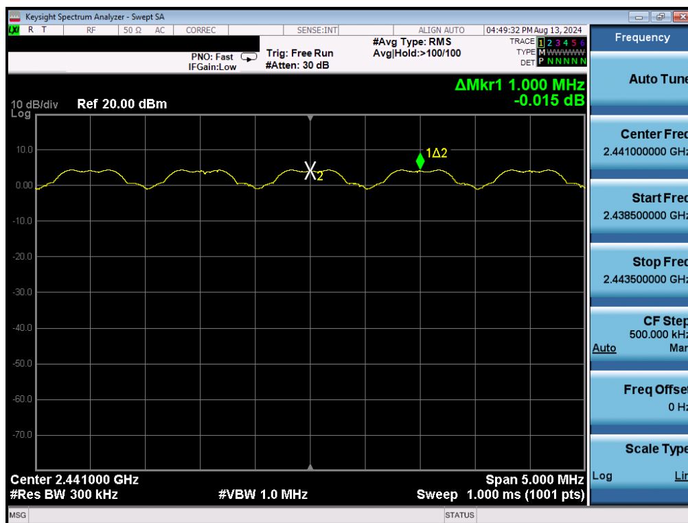
Plot 7-16. Channel Spacing Plot (Bluetooth, 8DPSK, iPA)
