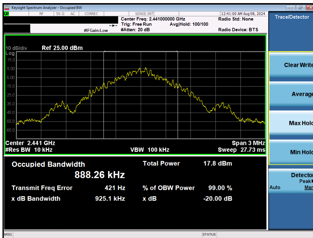
Plot 7-2. 20dB BW and 99% OBW Plot (Bluetooth, GFSK, iPA – Ch. 39)
