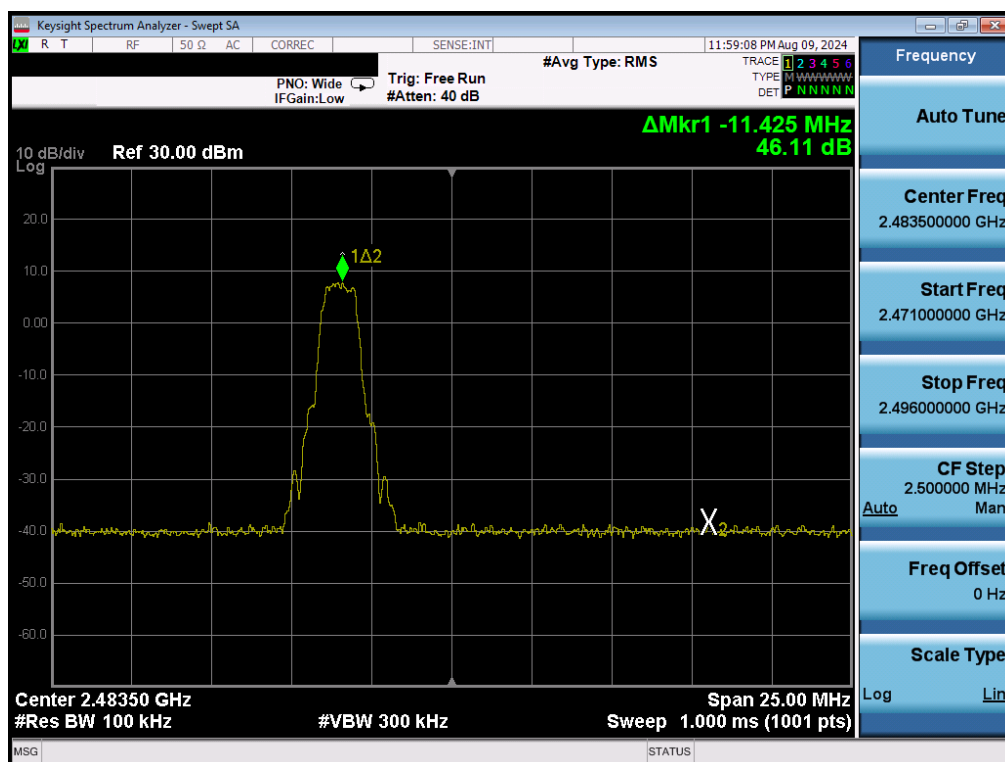
Plot 7-12. Band Edge Plot (Bluetooth with Hopping Disabled, 8DPSK, iPA – Ch. 78)
