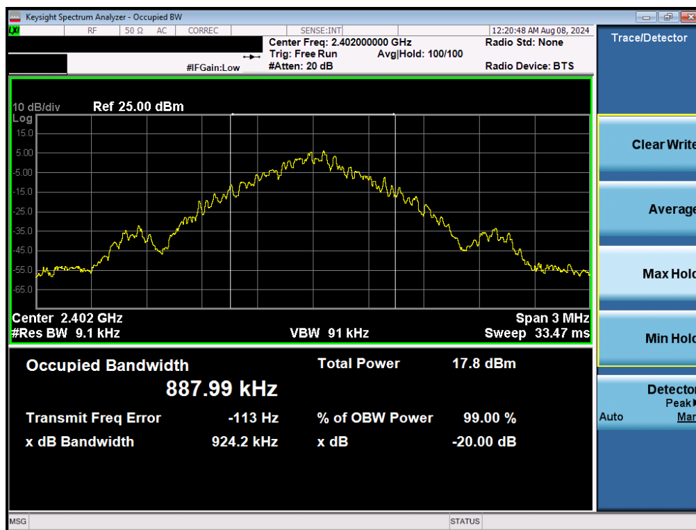
Plot 7-1. 20dB BW and 99% OBW Plot (Bluetooth, GFSK, iPA – Ch. 0)
