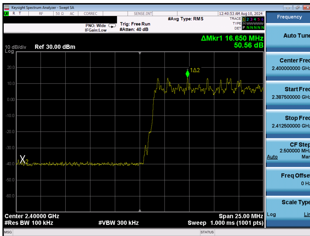
Plot 7-13. Band Edge Plot (Bluetooth with Hopping Enabled, 8DPSK, iPA)
