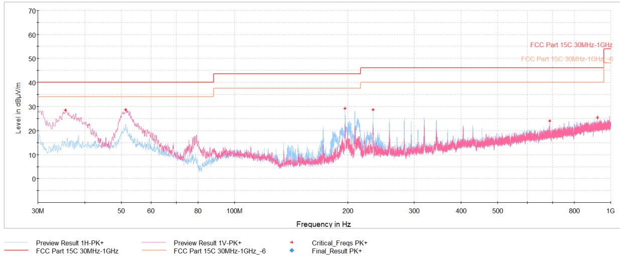
Plot 7-37. Radiated Spurious Emissions Below 1GHz (GFSK, iPA – Ch.78, with AC/DC adaptor via USB-C cable with wire charger)
