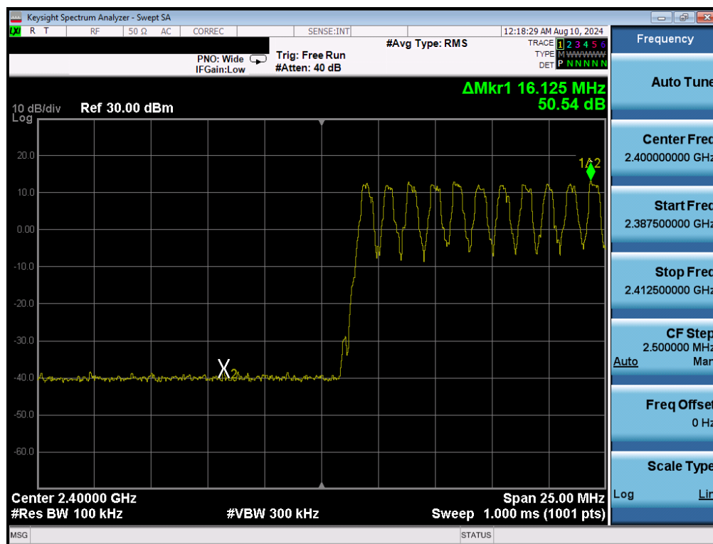
Plot 7-9. Band Edge Plot (Bluetooth with Hopping Enabled, GFSK, iPA)
