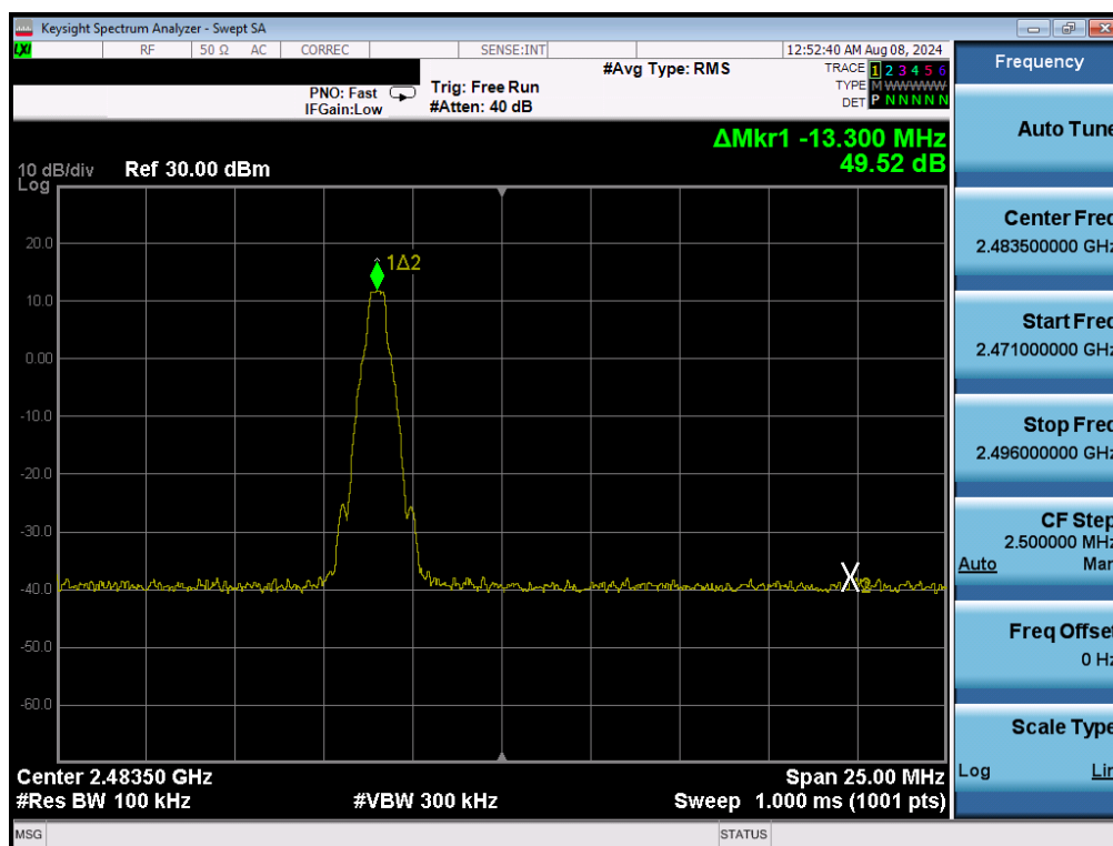
Plot 7-8. Band Edge Plot (Bluetooth with Hopping Disabled, GFSK, iPA – Ch. 78)
