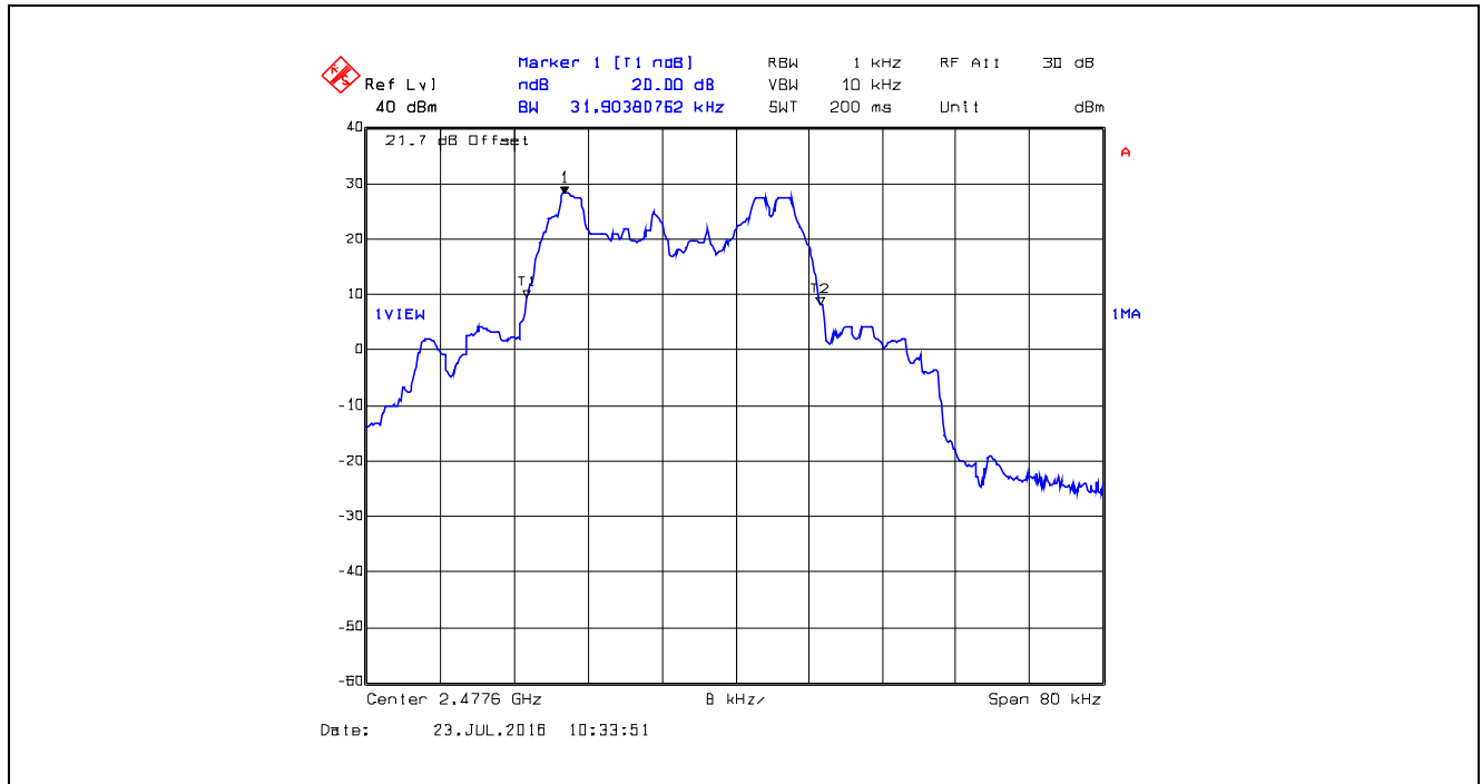
Plot 5.3.4.3. 20 dB Bandwidth, 2477.6 MHz, 24686 bps, 50 kHz CS, Power Scheme Raw, Raw Power 63
