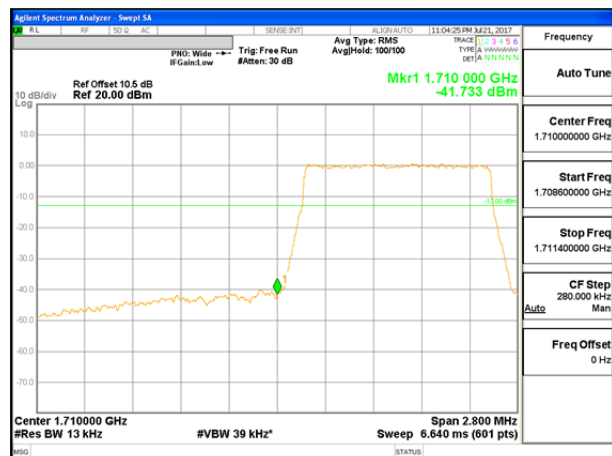
LTE B66 1.4MHz 16QAM Low Channel FRB
