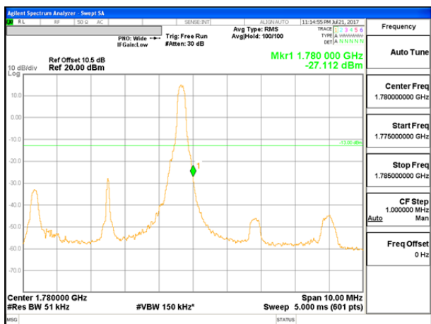
LTE B66 5MHz QPSK High Channel 1RB
