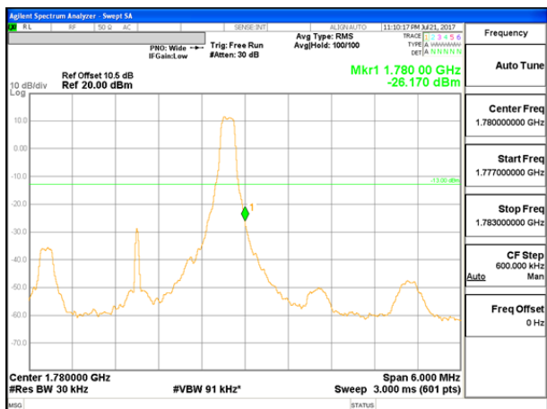
LTE B66 3MHz 16QAM High Channel 1RB
