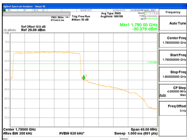
LTE B66 20MHz 16QAM High Channel FRB
