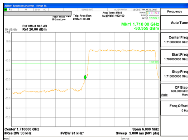
LTE B66 3MHz QPSK Low Channel 1RB
