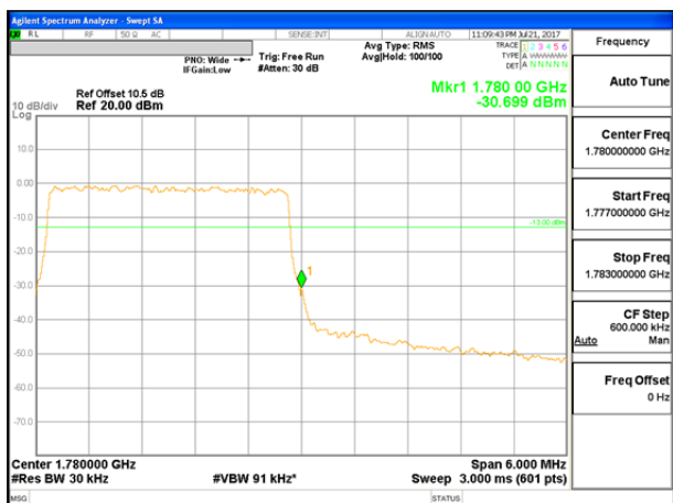
LTE B66 3MHz 16QAM High Channel FRB
