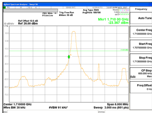
LTE B66 3MHz 16QAM Low Channel 1RB
