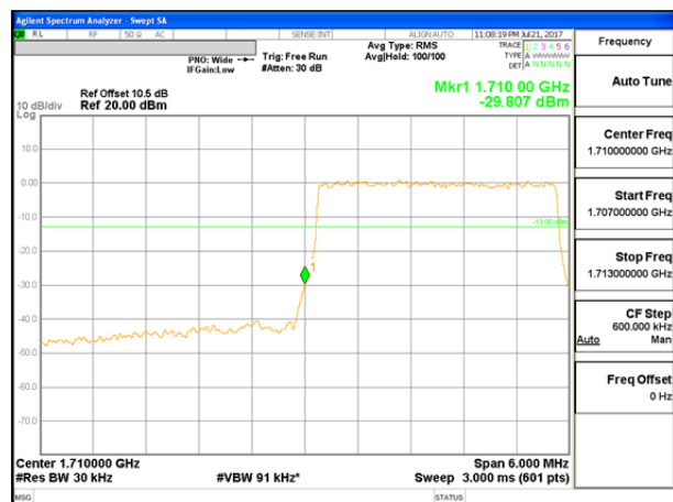
LTE B66 3MHz 16QAM Low Channel FRB
