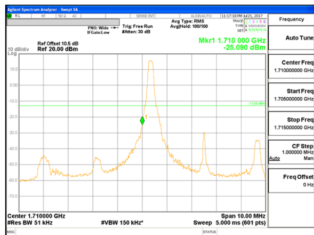
LTE B66 5MHz QPSK Low Channel 1RB
