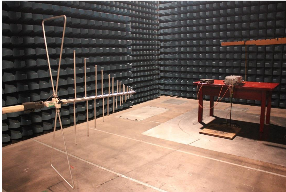
Transmitting Spurious emission ( below 1GHz)
