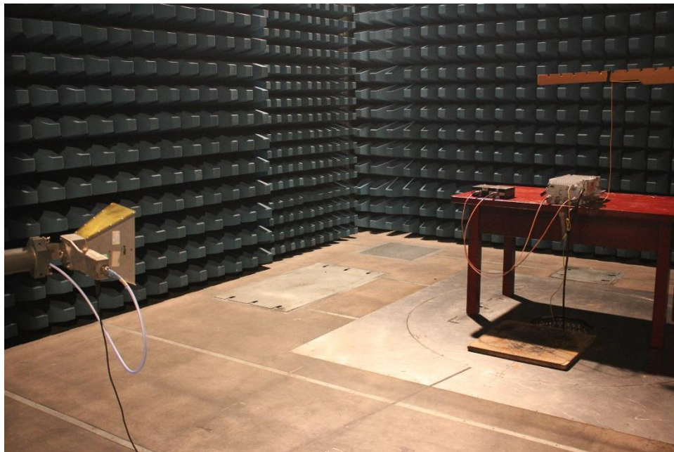
Transmitting Spurious emission ( Above 1GHz)
