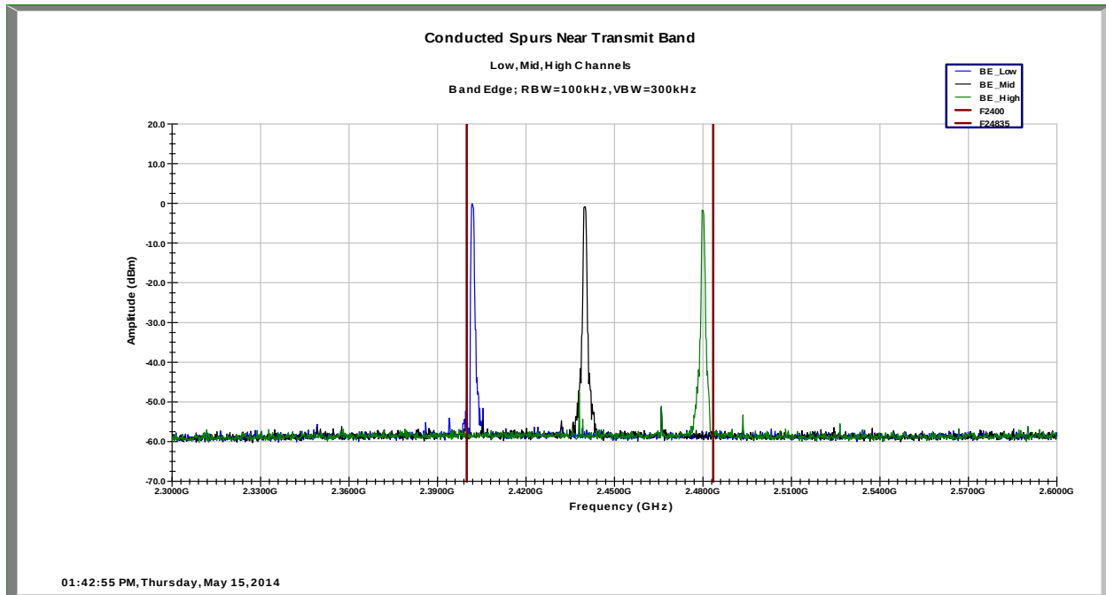
Low / High Band Edge Plot
