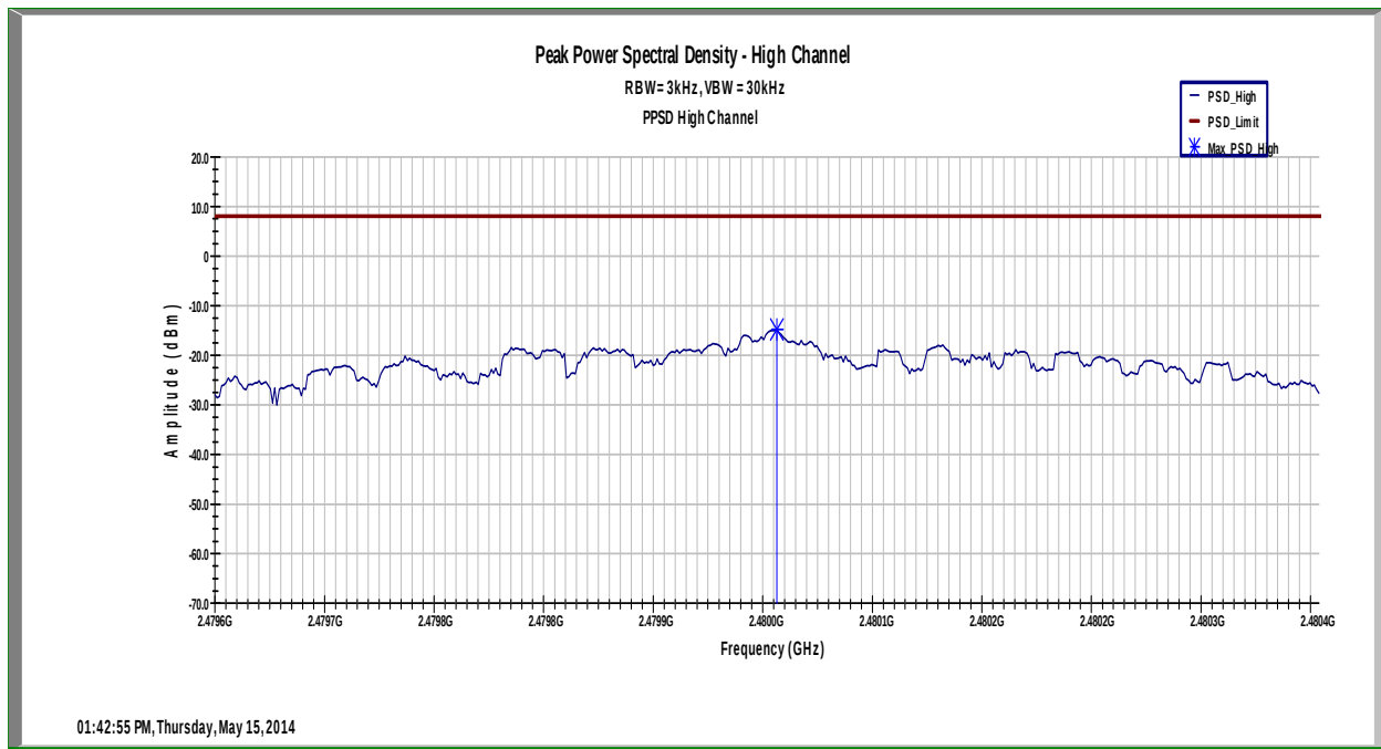
PPSD, High Channel
