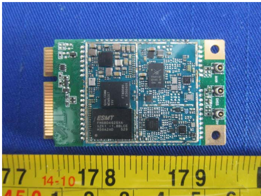
EUT - Top Cover off View (EC21-A MINIPCIE)
