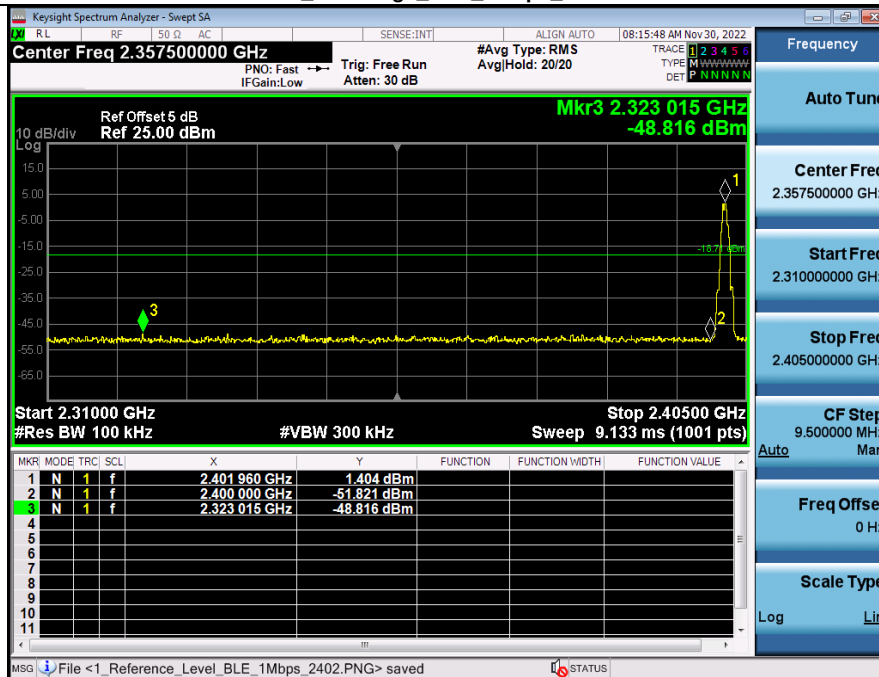
2 Bandedge_BLE_1Mbps_2402
