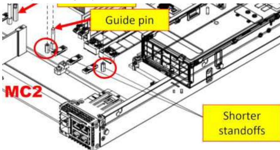
Figure 45. VEP4600 WIFI carrier card guide pin and shorter standoffs
