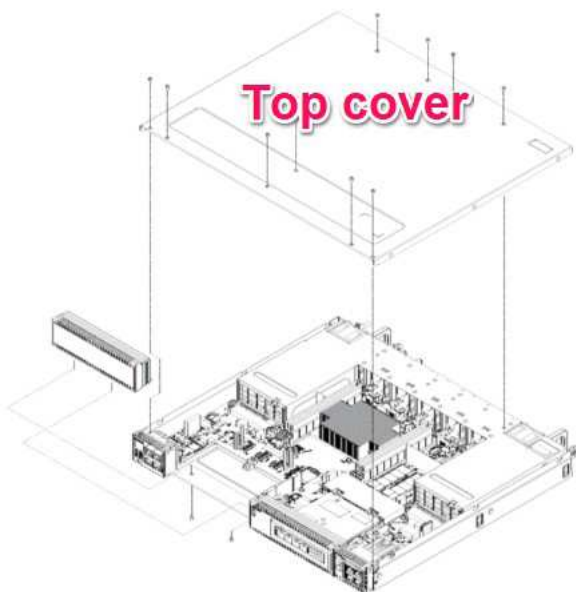
Figure 51. Place the top cover back on the unit
