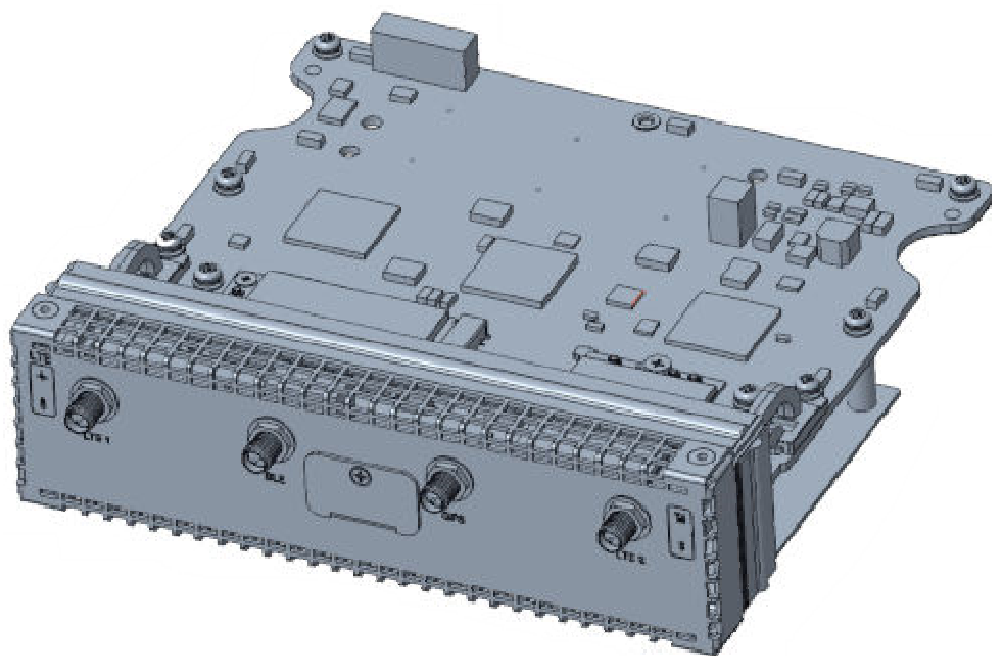
Figure 46. LTE card without antennas
