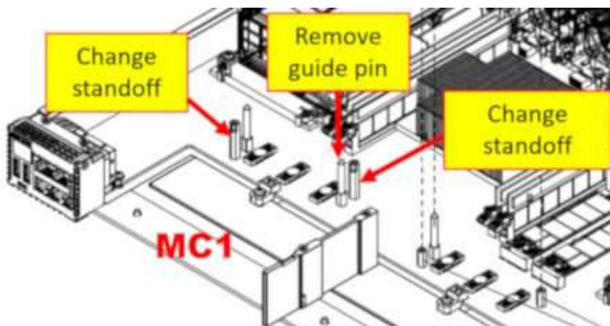
Figure 44. Change standoffs
