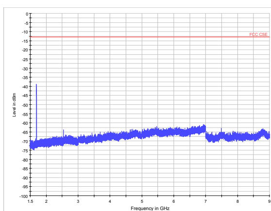
LTE Band 5 1.4MHz CH-High 1.5GHz~9GHz
