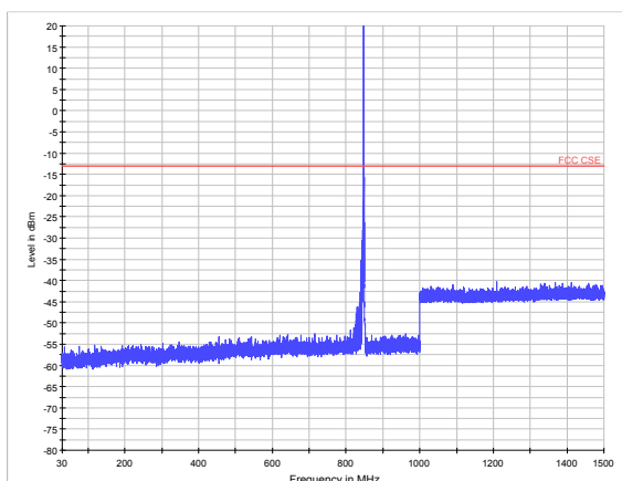
LTE Band 5 1.4MHz CH-High 30MHz~1.5GHz
