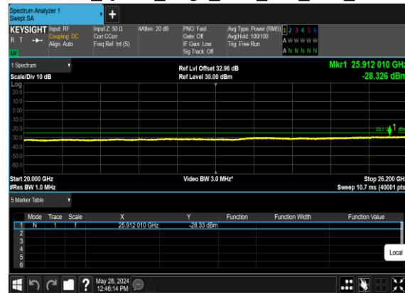
N38(25M)_DFT-s- OFDM_QPSK_Edge_1RB_Left_Low_CH
