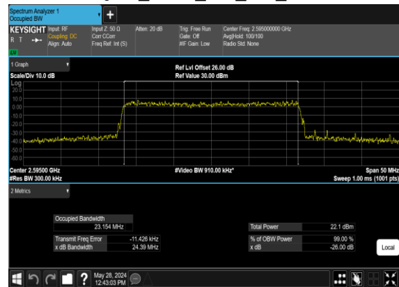
N38(25M)_CP-OFDM_256 QAM_Outer_Full_Mid_CH
