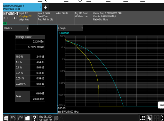
N41(20M)_DFT-s-OFDM_QPSK_Edge_1RB_Left_Mid_CH
