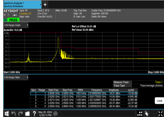
N38(25M)_DFT-s- OFDM_QPSK_Edge_1RB_Right_High_CH
