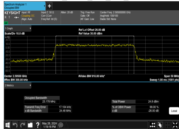
N38(25M)_CP-OFDM_16 QAM_Outer_Full_Mid_CH
