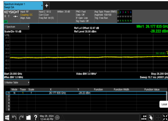
N38(25M)_DFT-s- OFDM_BPSK_Edge_1RB_Left_Low_CH
