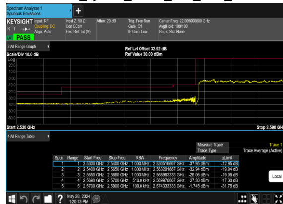
N38(25M)_DFT-s-OFDM_QPSK_Outer_Full_Low_CH
