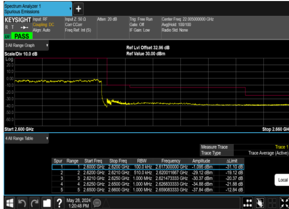
N38(25M)_DFT-s- OFDM_BPSK_Outer_Full_High_CH
