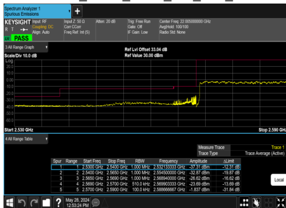
N38(25M)_DFT-s-OFDM_BPSK_Outer_Full_Low_CH
