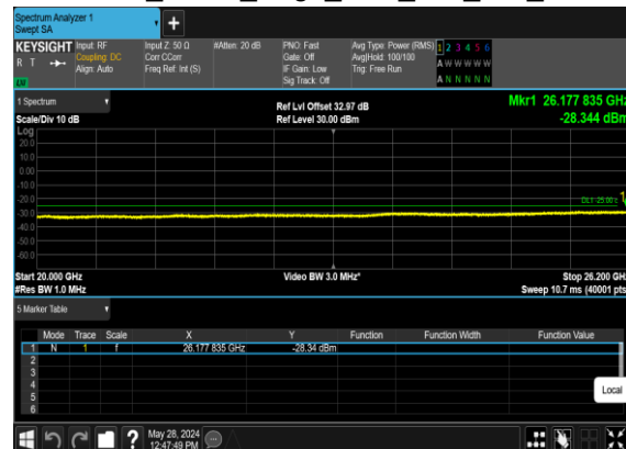
N38(25M)_DFT-s- OFDM_BPSK_Edge_1RB_Left_Mid_CH
