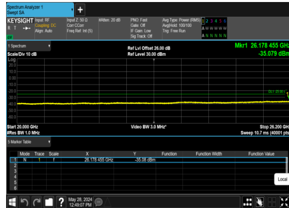
N38(25M)_DFT-s- OFDM_QPSK_Edge_1RB_Left_Mid_CH
