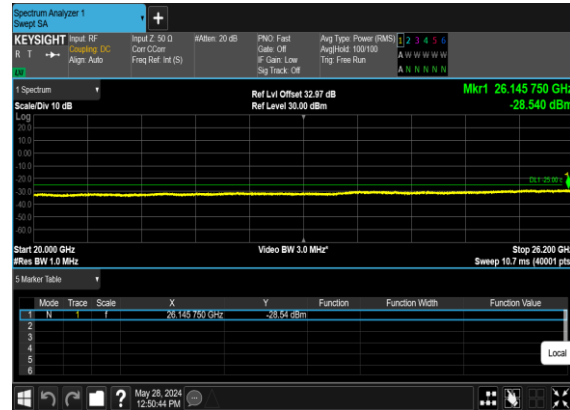
N38(25M)_DFT-s- OFDM_BPSK_Edge_1RB_Left_High_CH
