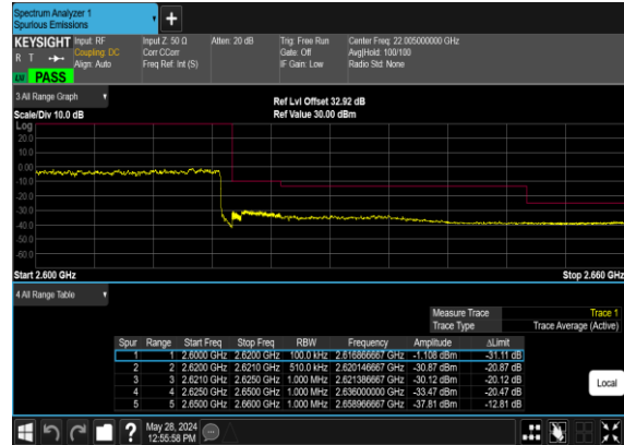
N38(25M)_DFT-s- OFDM_QPSK_Outer_Full_High_CH
