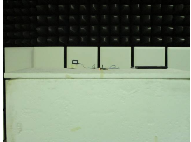
FCC_15_247_902~928MHz_OFDM_Radiated_Monopole_Setup
