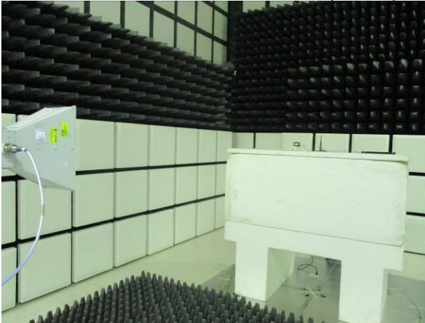
FCC_15_247_902~928MHz_OFDM_Radiated_Dipole_Setup
