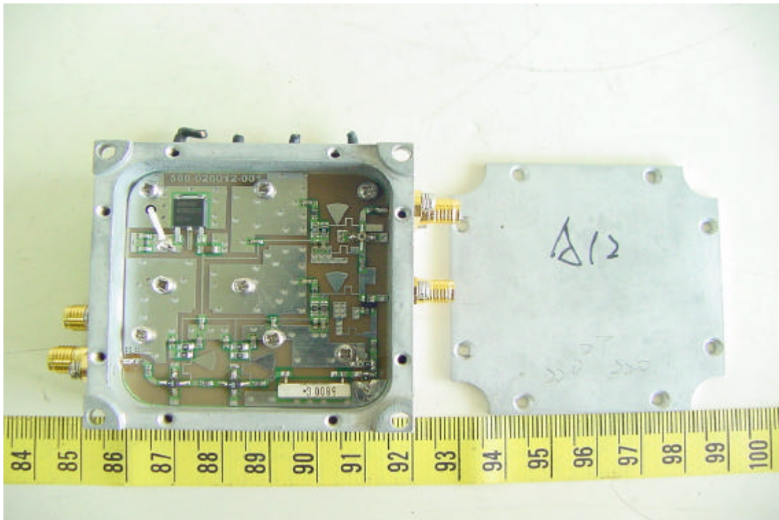
41. Internal View of EUT
