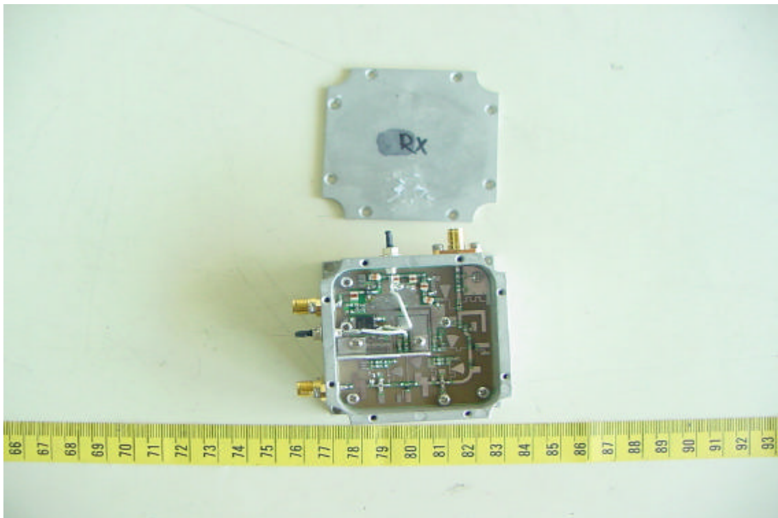
42. Internal View of EUT
