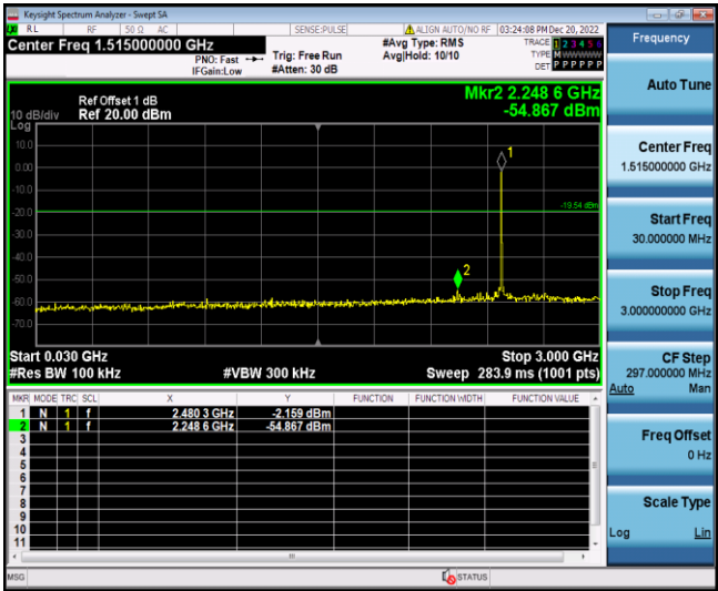
BLE_2Mbps_Ant1_2480_30~3000
