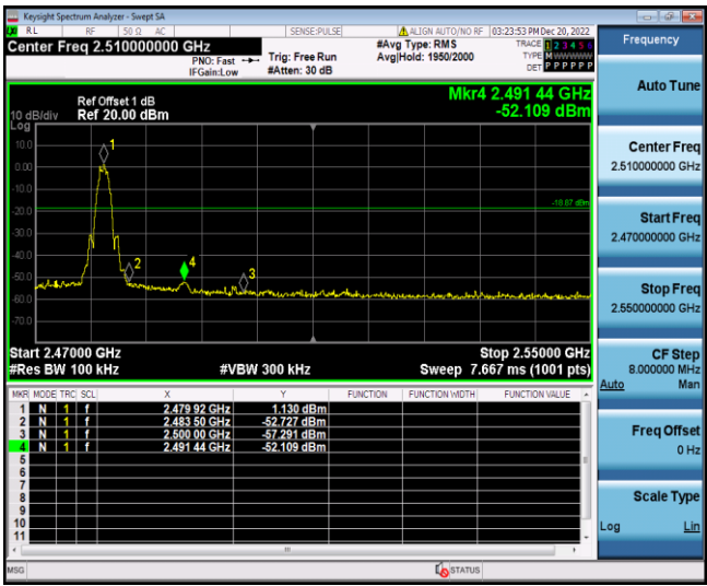
BLE_2Mbps_Ant1_High_2480
