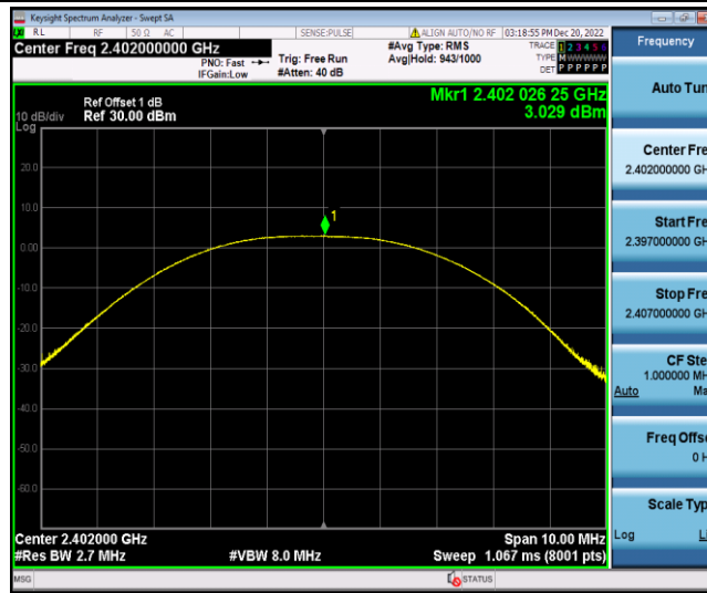
BLE_2Mbps_Ant1_2402
