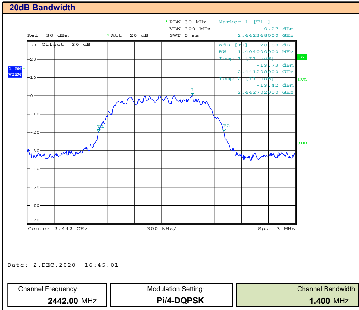
Plot 14.2 – BT ERD 2MB 20dB BW
