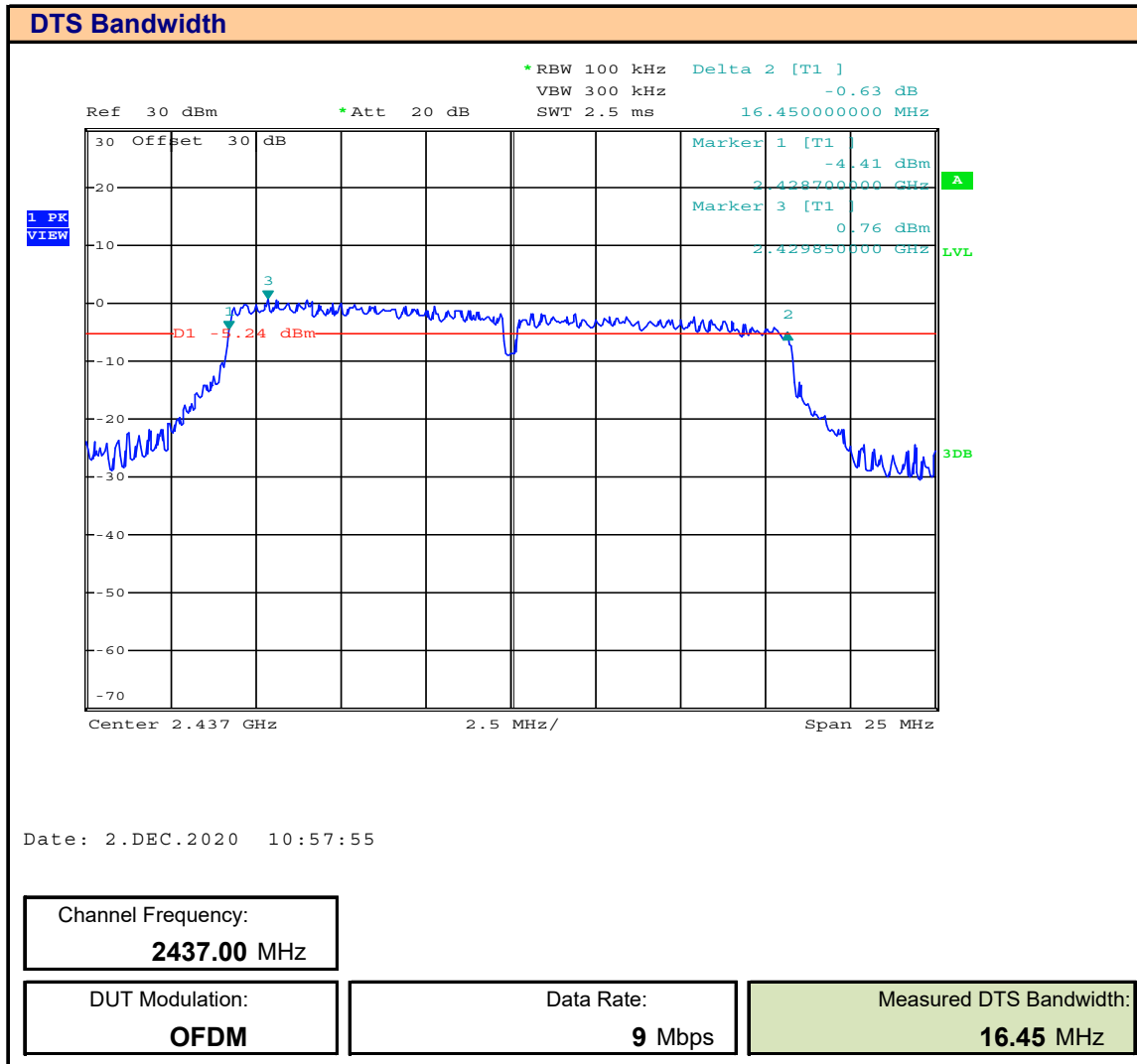
Plot 8.3 – 6dB DTS Bandwidth 802.11g
