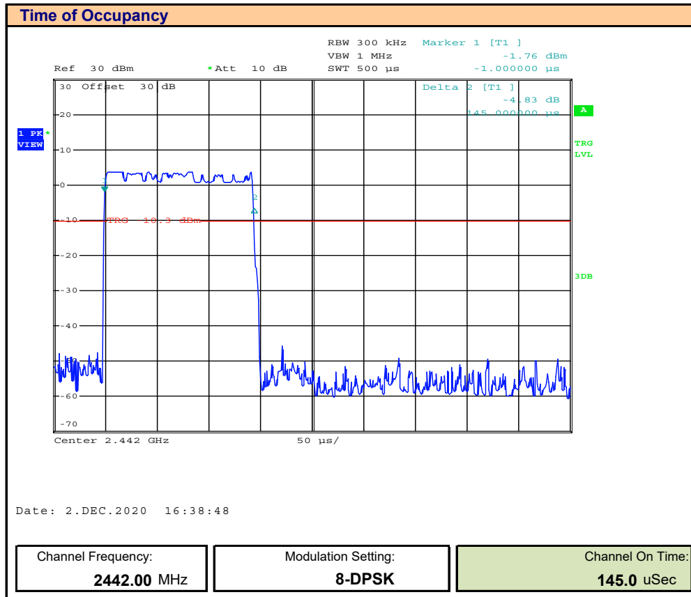
Plot 15.2 – Time of Occupancy, BT EDR 3MB
