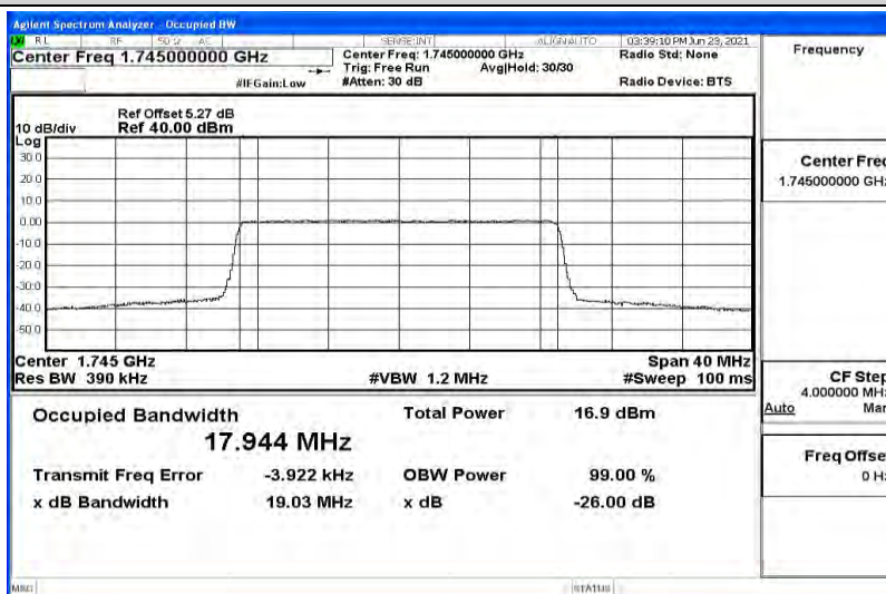
Band4-20MHz-16QAM-20300-100RB#0-17.944
