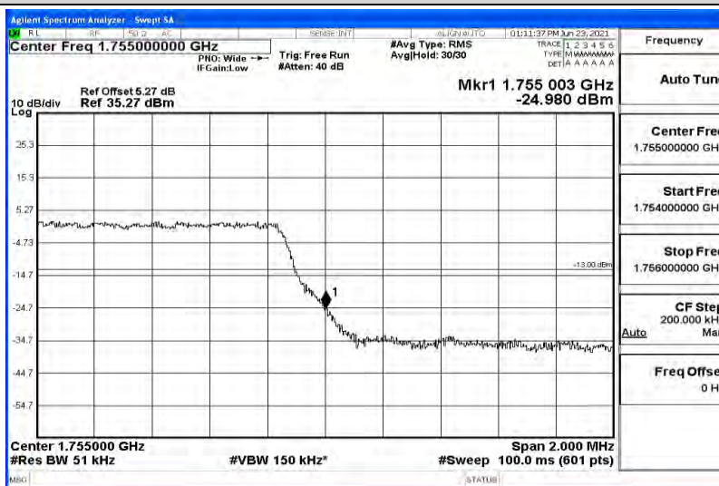
Band4-5MHz-QPSK-19975-25RB#0
