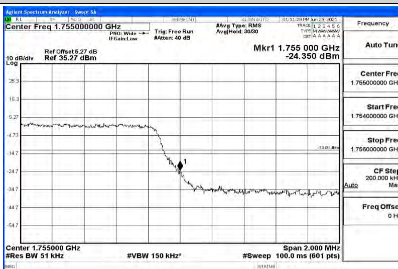
Band4-3MHz-16QAM-19965-15RB#0
