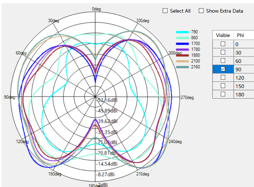
DCS1800/WCDMA B4/ LTEB3/B4/B20 Phi=90deg
