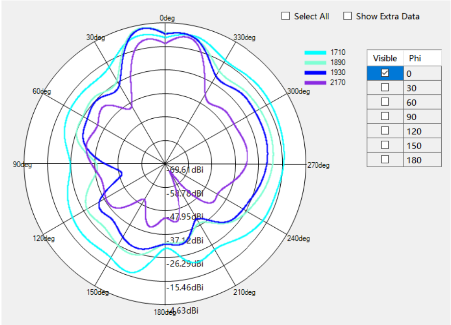
DCS1800/PCS1900/WCDMA B1/B2/B4/LTE B1/2/3/4 \Phi=0^\circ
