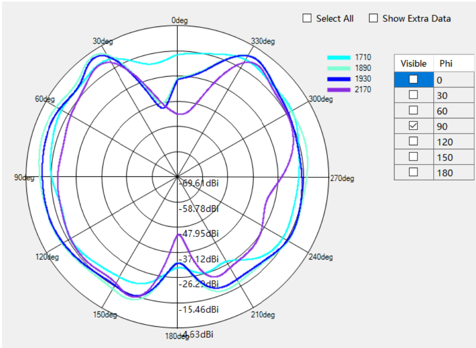
DCS1800/PCS1900/WCDMA B1/B2/B4/LTE B1/2/3/4 \Phi=90^\circ
