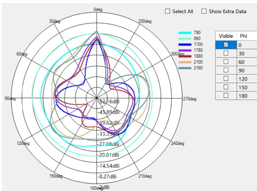
DCS1800/WCDMA B4/ LTEB3/B4/B20Phi=0deg
