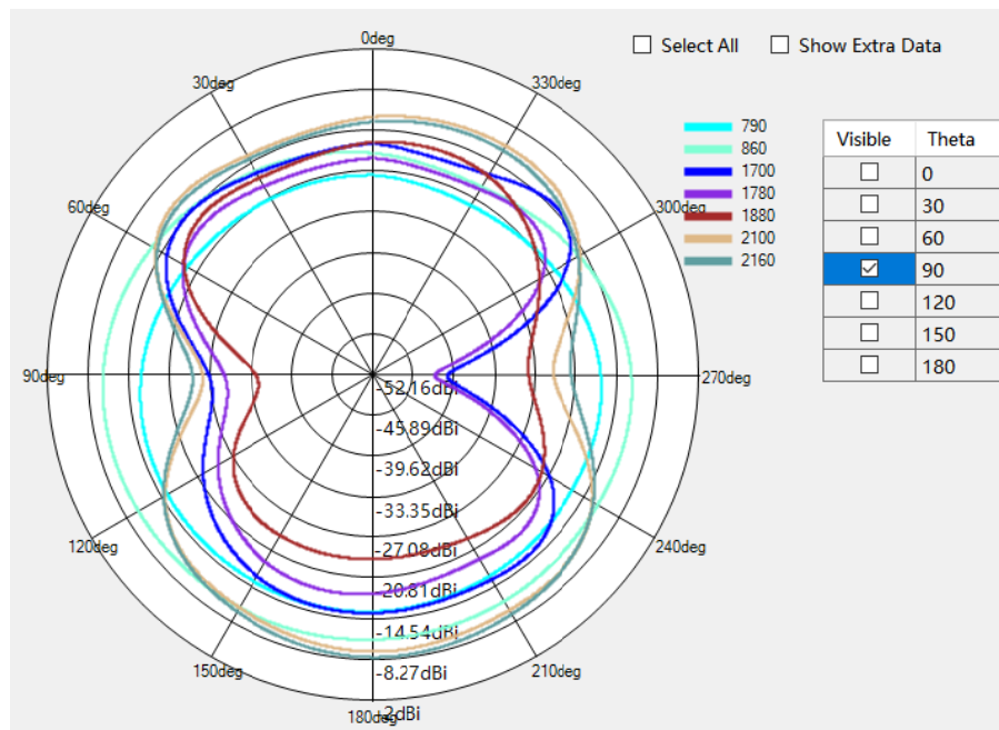
DCS1800/WCDMA B4/ LTEB3/B4/B20 Theta=90deg
