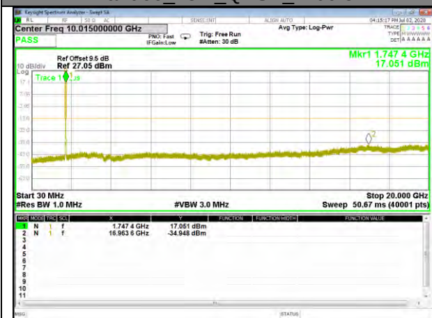
Band66_15M_QPSK_Middle
