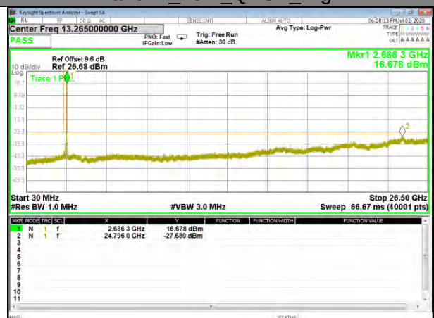
Band41_15M_QPSK_High
