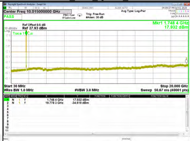
Band66_15M_QPSK_Low
