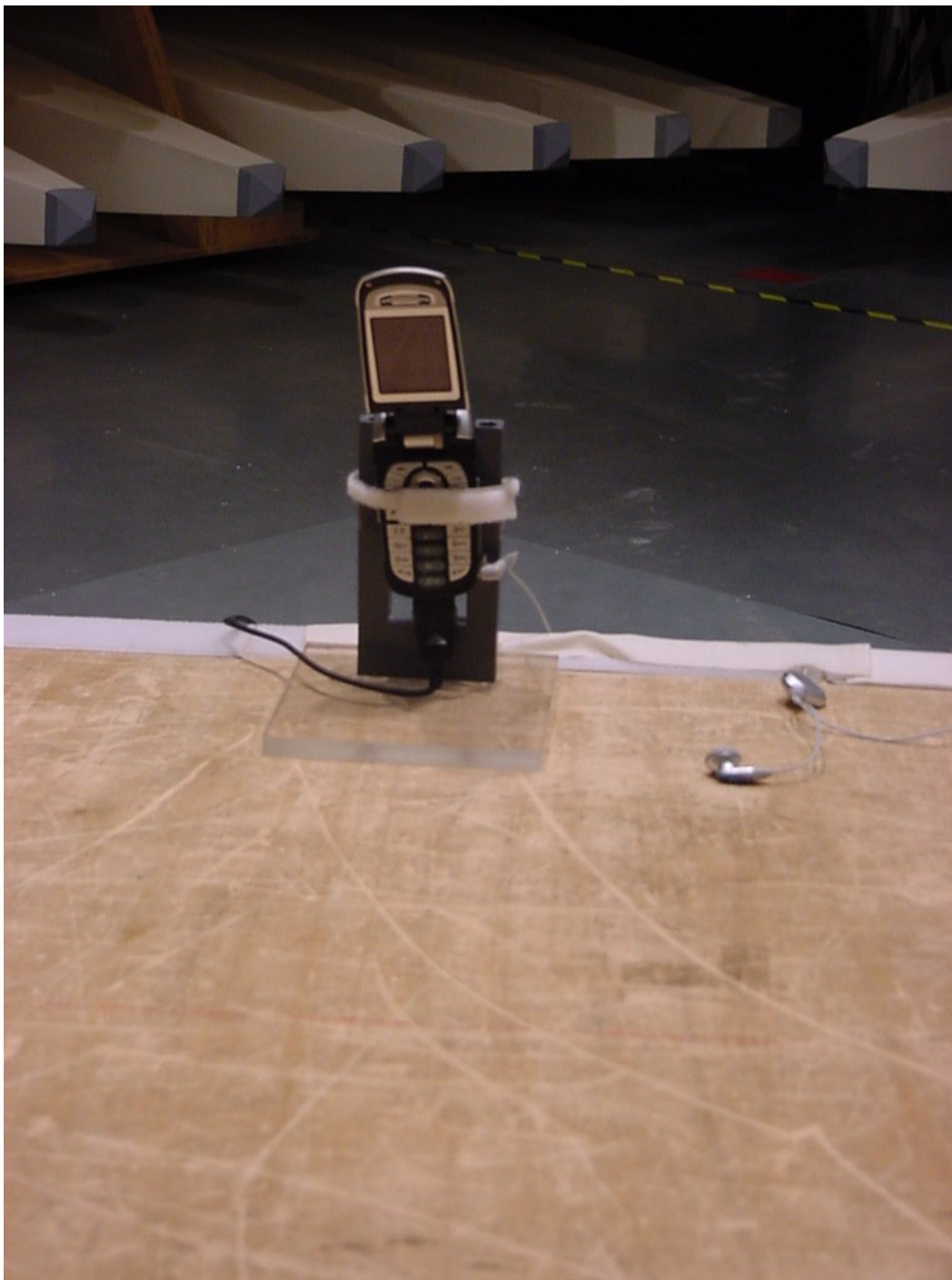
Photo 1 (Radiated Emissions): Test set-up I
