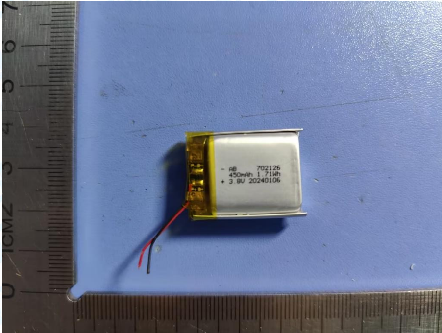
Photo 8 Battery appearance
