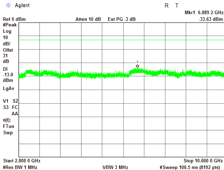
Plot 7.4.20 Spurious emission measurements in 2800 - 10000 MHz at mid carrier frequency
