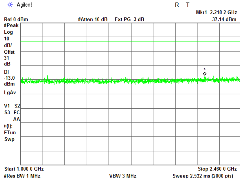
Plot 7.4.12 Spurious emission measurements in 1000 - 2460 MHz at mid carrier frequency
