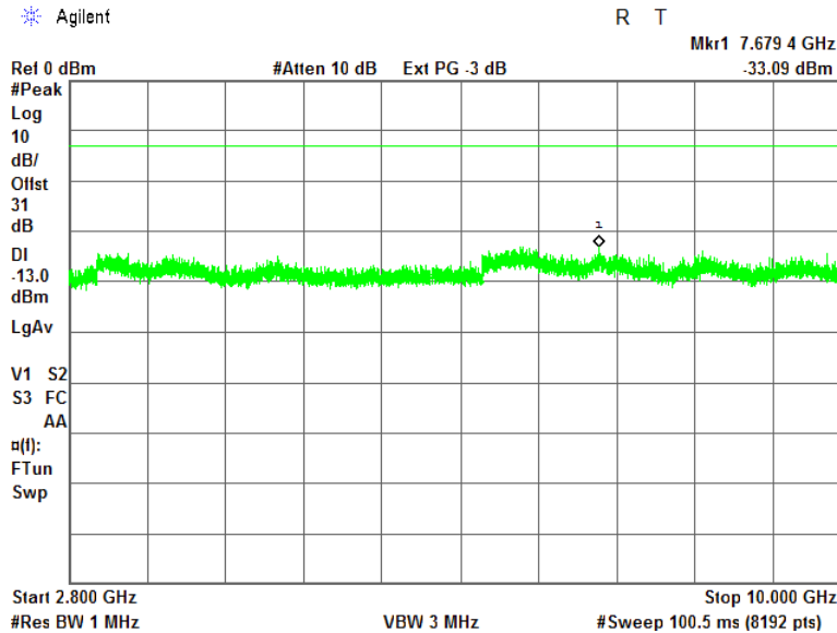
Plot 7.4.19 Spurious emission measurements in 2800-10000 MHz range at low carrier frequency
