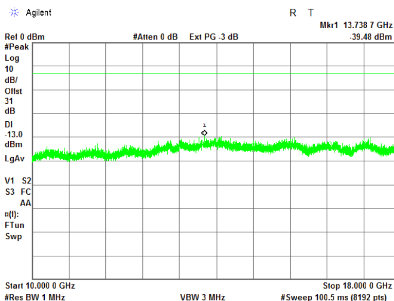
Plot 7.4.24 Spurious emission measurements in 10000 - 18000 MHz at high carrier frequency
