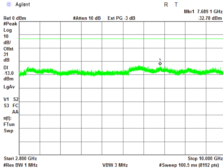
Plot 7.4.21 Spurious emission measurements in 2800 - 10000 MHz at high carrier frequency
