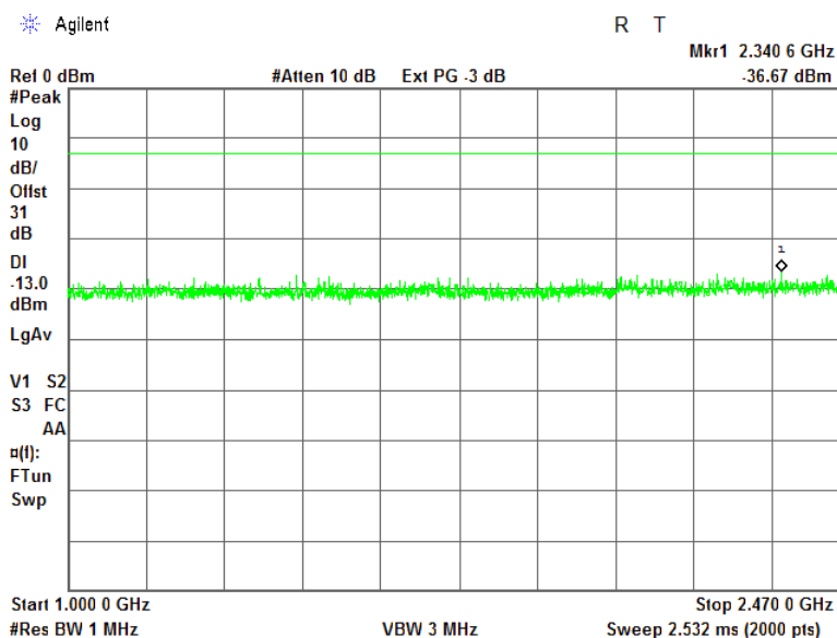
Plot 7.4.10 Spurious emission measurements in 1000 - 2470 MHz range at low carrier frequency
