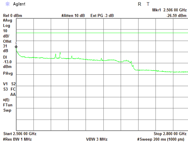
Plot 7.4.16 Spurious emission measurements in 2506 - 2800 MHz range at low carrier frequency
