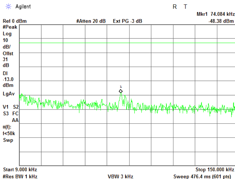
Plot 7.4.1 Spurious emission measurements in 9 - 150 kHz range at low carrier frequency
