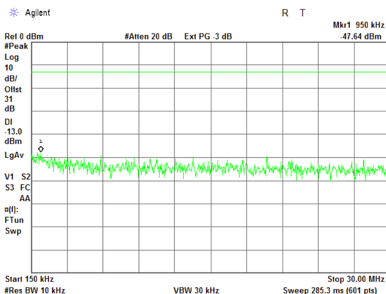
Plot 7.4.6 Spurious emission measurements in 0.15 - 30.0 MHz range at high carrier frequency
