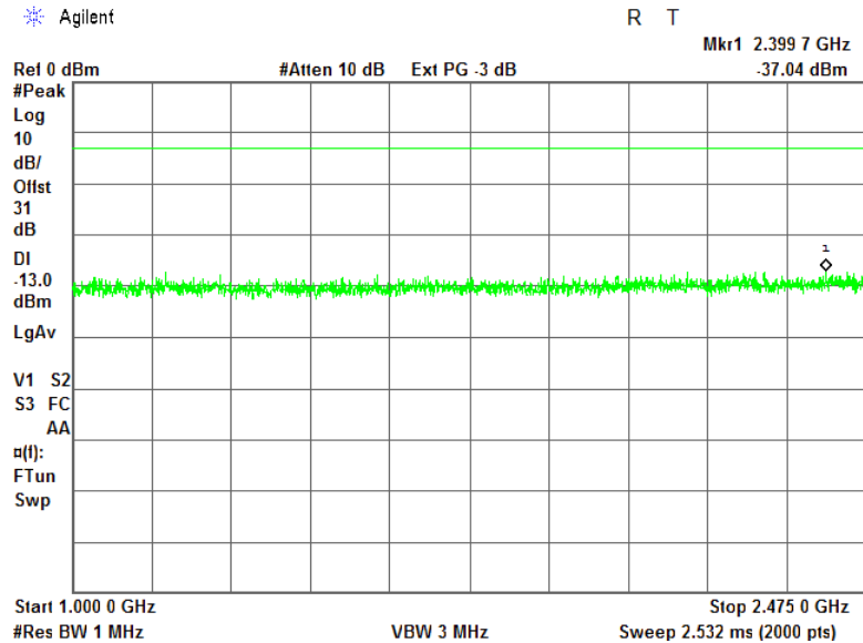
Plot 7.4.14 Spurious emission measurements in 1000 - 2475 MHz at high carrier frequency
