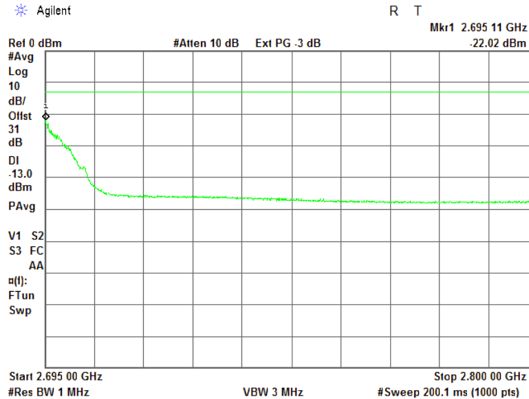
Plot 7.4.18 Spurious emission measurements in 2695 - 2800 MHz at high carrier frequency
