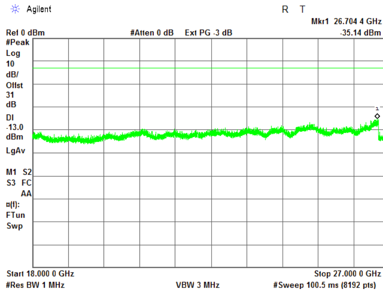
Plot 7.4.25 Spurious emission measurements in 18000-27000 MHz range at low carrier frequency
