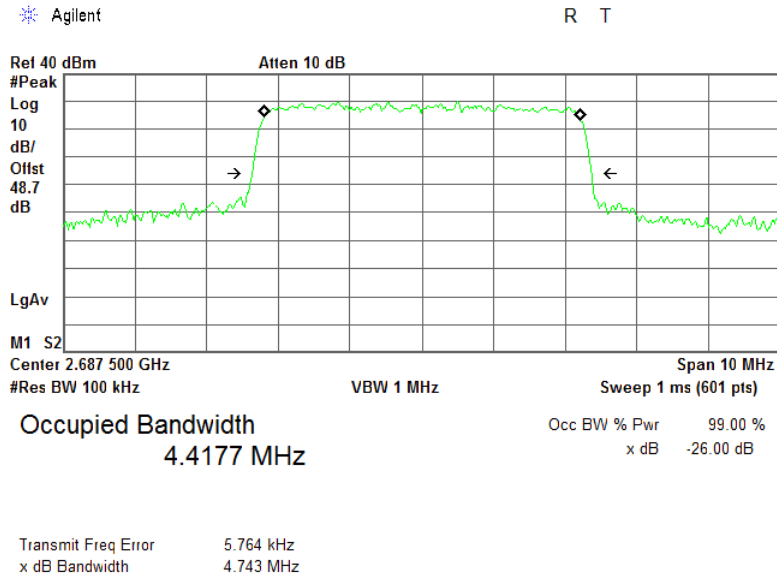
Plot 7.1.3 Occupied bandwidth test results at high frequency, 5 MHz EBW, QPSK, RF#2
