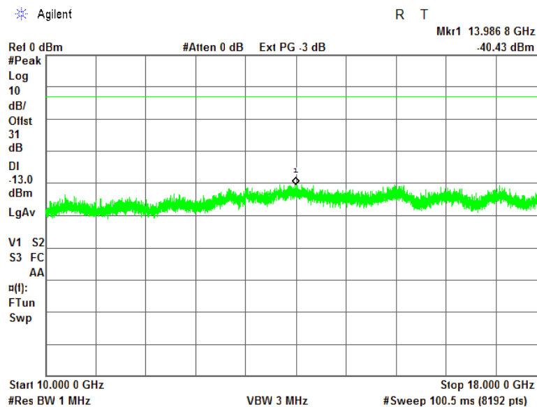
Plot 7.4.22 Spurious emission measurements in 10000-18000 MHz range at low carrier frequency
