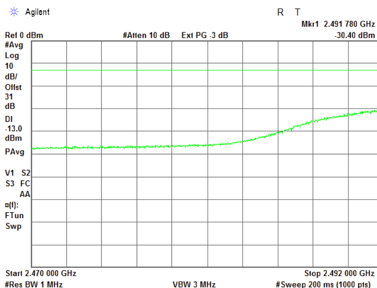
Plot 7.4.11 Spurious emission measurements in 2470 – 2492 MHz range at low carrier frequency
