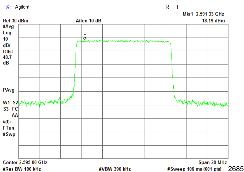
Plot 7.2.20 Power spectral density test results at mid frequency, QPSK, 10 MHz EBW, RF # 2
