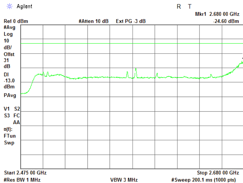
Plot 7.4.15 Spurious emission measurements in 2475 -2680 MHz at high carrier
