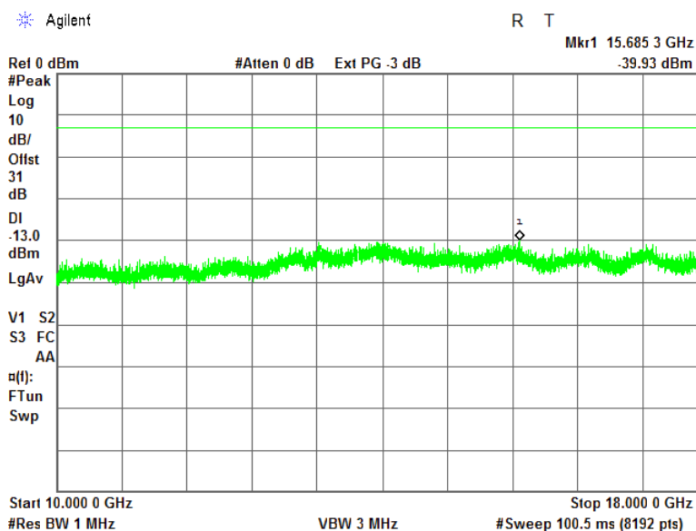
Plot 7.4.23 Spurious emission measurements in 10000 - 18000 MHz at mid carrier frequency
