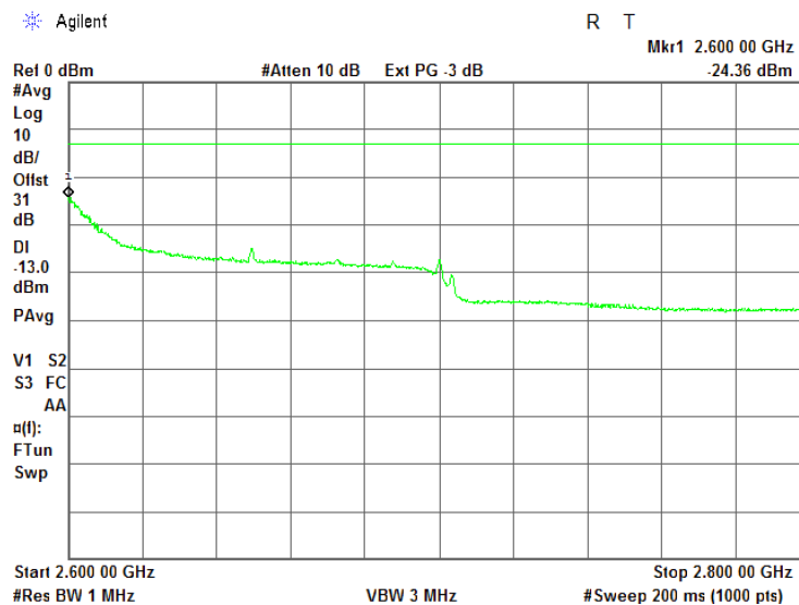
Plot 7.4.17 Spurious emission measurements in 2600 - 2800 MHz at mid carrier frequency
