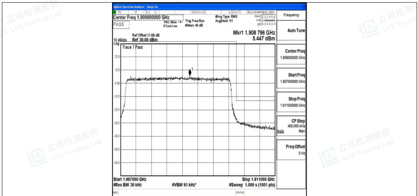
Band2_3MHz_QPSK_19185_15RB#0
