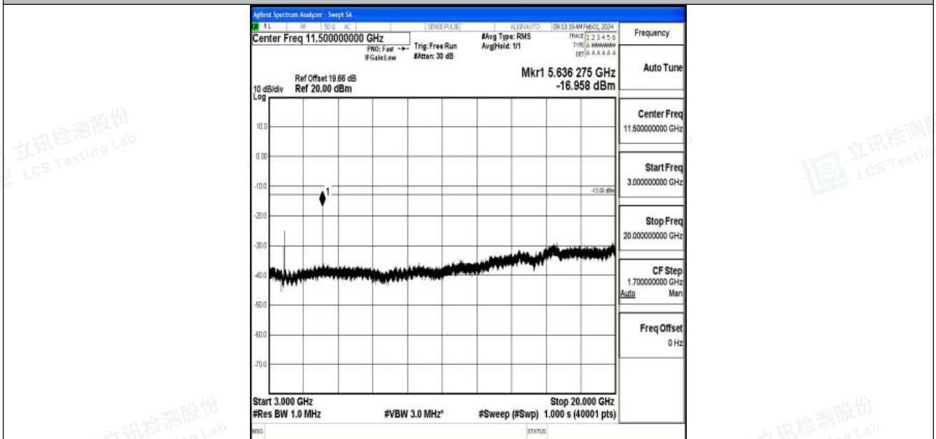
Band2_3MHz_16QAM_18900_1RB#0_3000~20000_3000~20000
