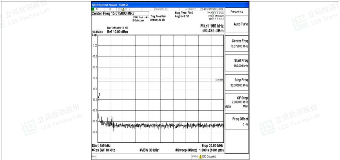
Band2_1.4MHz_16QAM_18900_1RB#0_0.15~30_0.15~30
