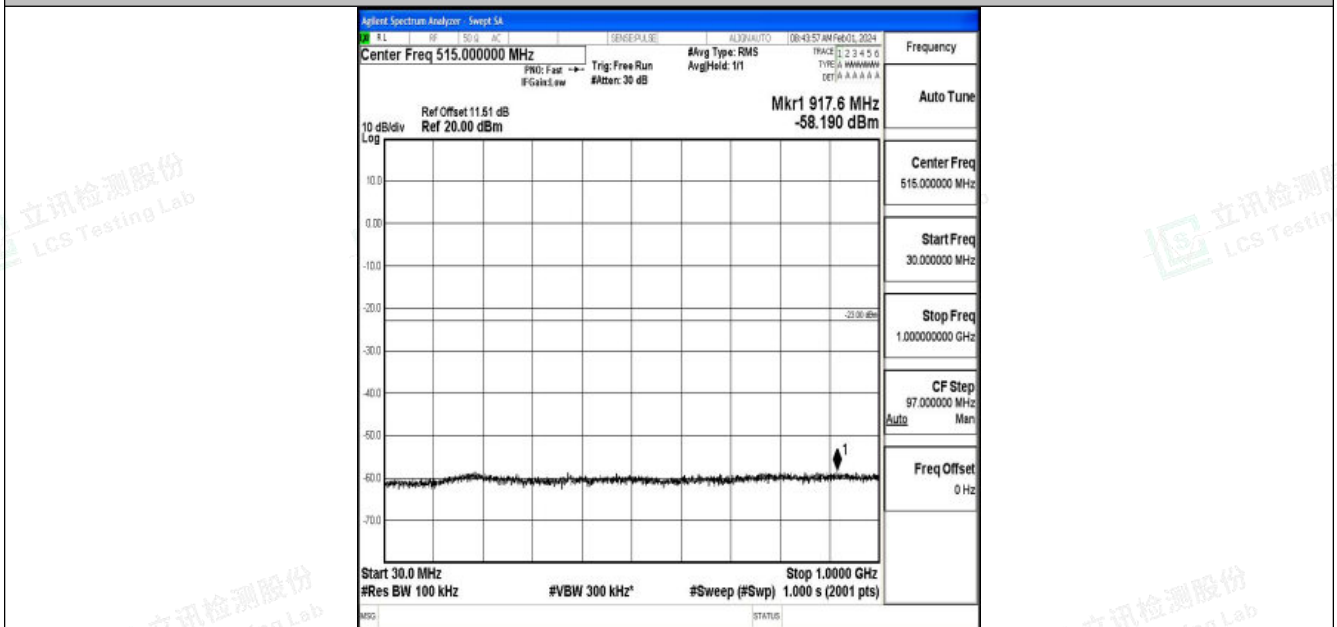
Band2_1.4MHz_16QAM_18900_1RB#0_30~1000_30~1000
