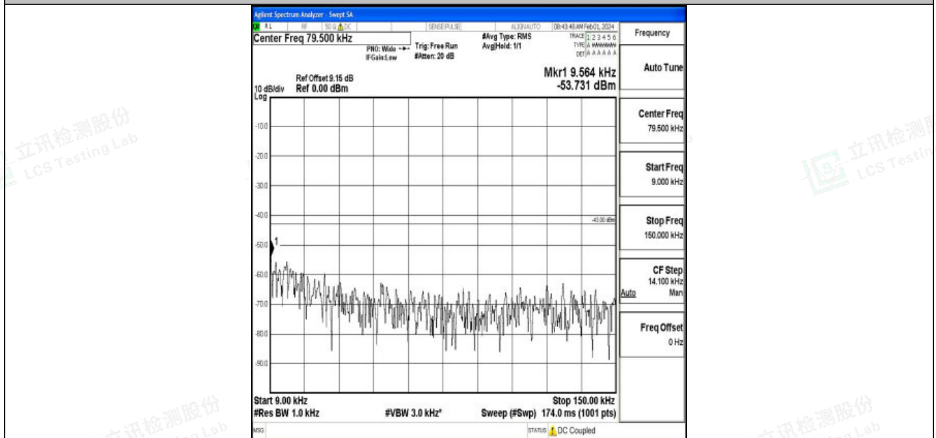
Band2_1.4MHz_16QAM_18900_1RB#0_0.009~0.15_0.009~0.15
