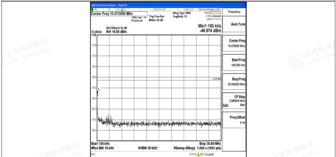
Band2_1.4MHz_QPSK_19193_1RB#0_0.15~30_0.15~30
