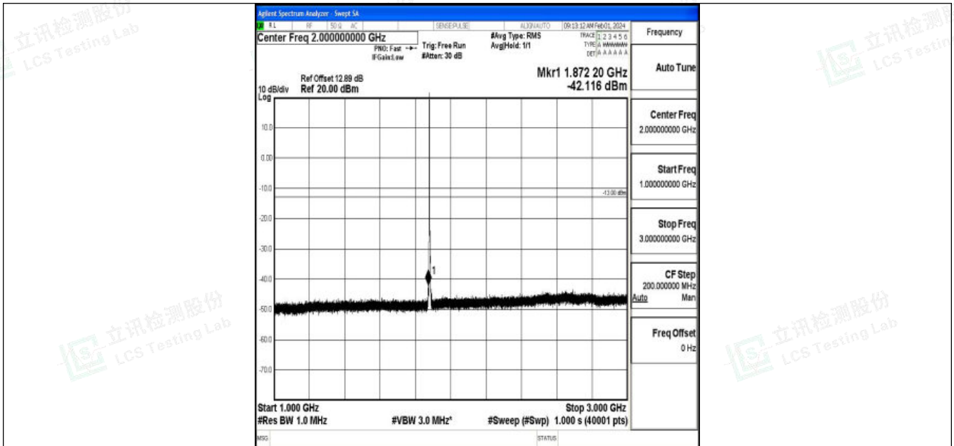
Band2_3MHz_16QAM_18900_1RB#0_1000~3000_1000~3000
