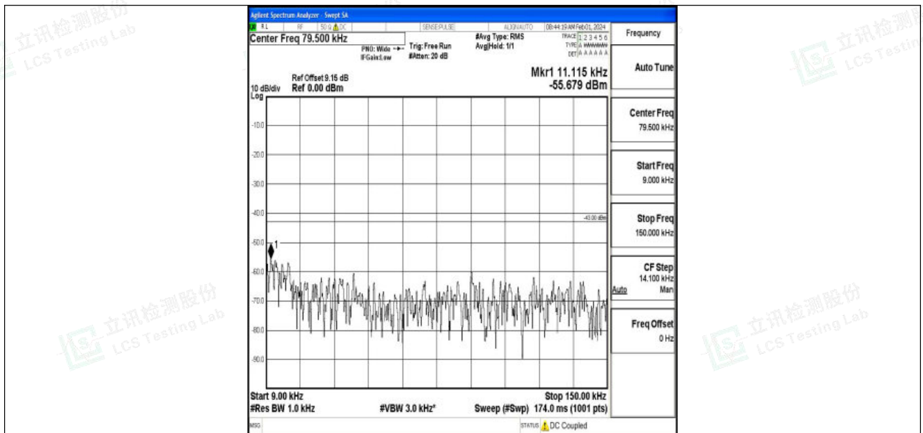
Band2_1.4MHz_QPSK_19193_1RB#0_0.009~0.15_0.009~0.15
