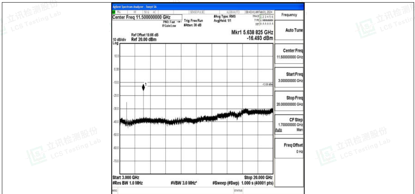
Band2_1.4MHz_QPSK_18900_1RB#0_3000~20000_3000~20000
