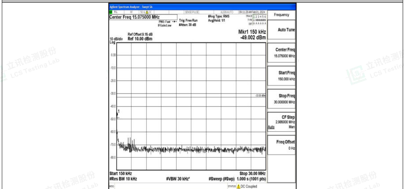
Band2_3MHz_QPSK_18615_1RB#0_0.15~30_0.15~30
