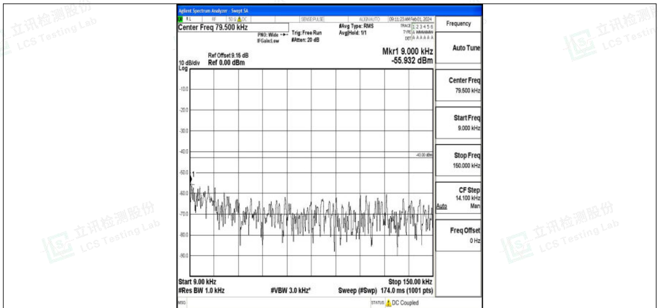
Band2_3MHz_QPSK_18615_1RB#0_0.009~0.15_0.009~0.15
