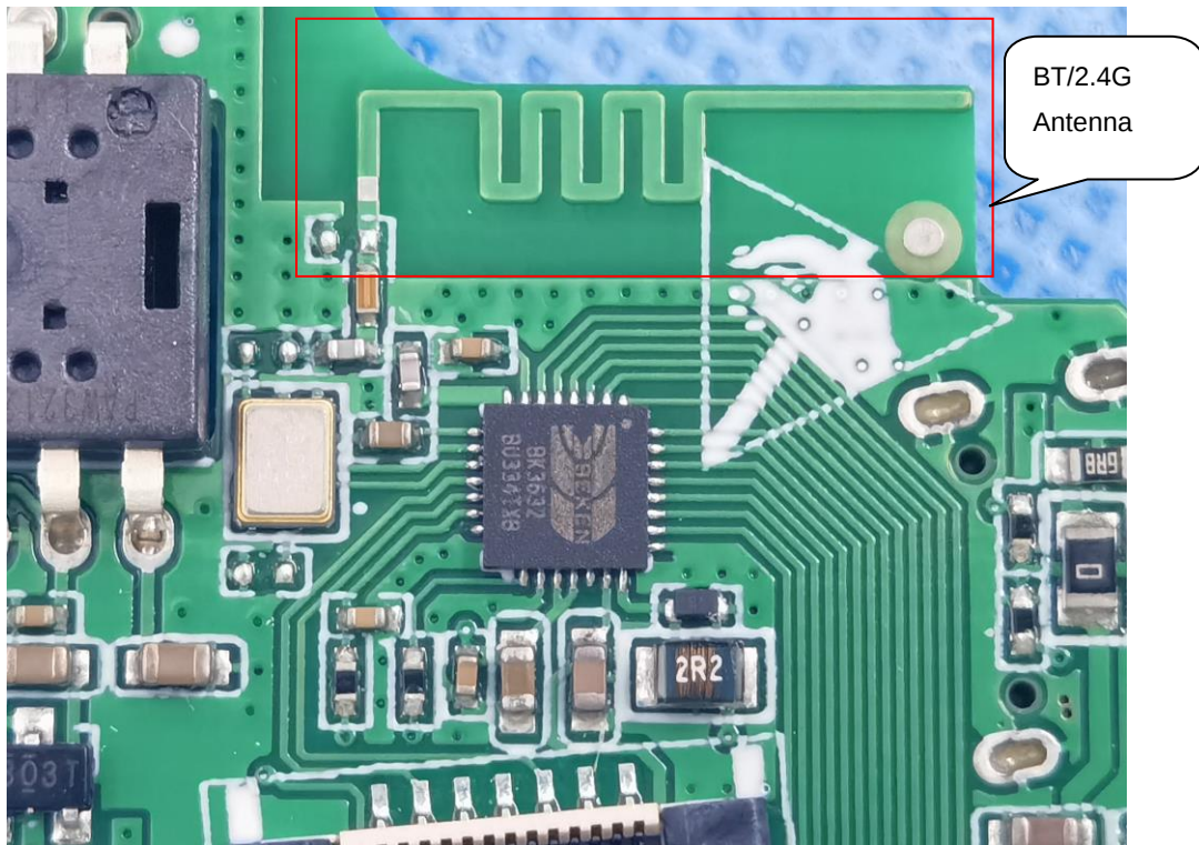
INTERNAL VIEW OF EUT (FIGURE 9)
