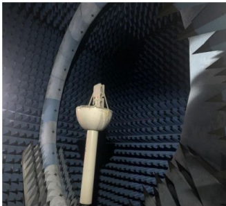
Chamber setup
