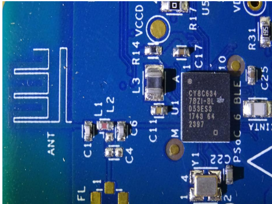
Radio part with Antenna
